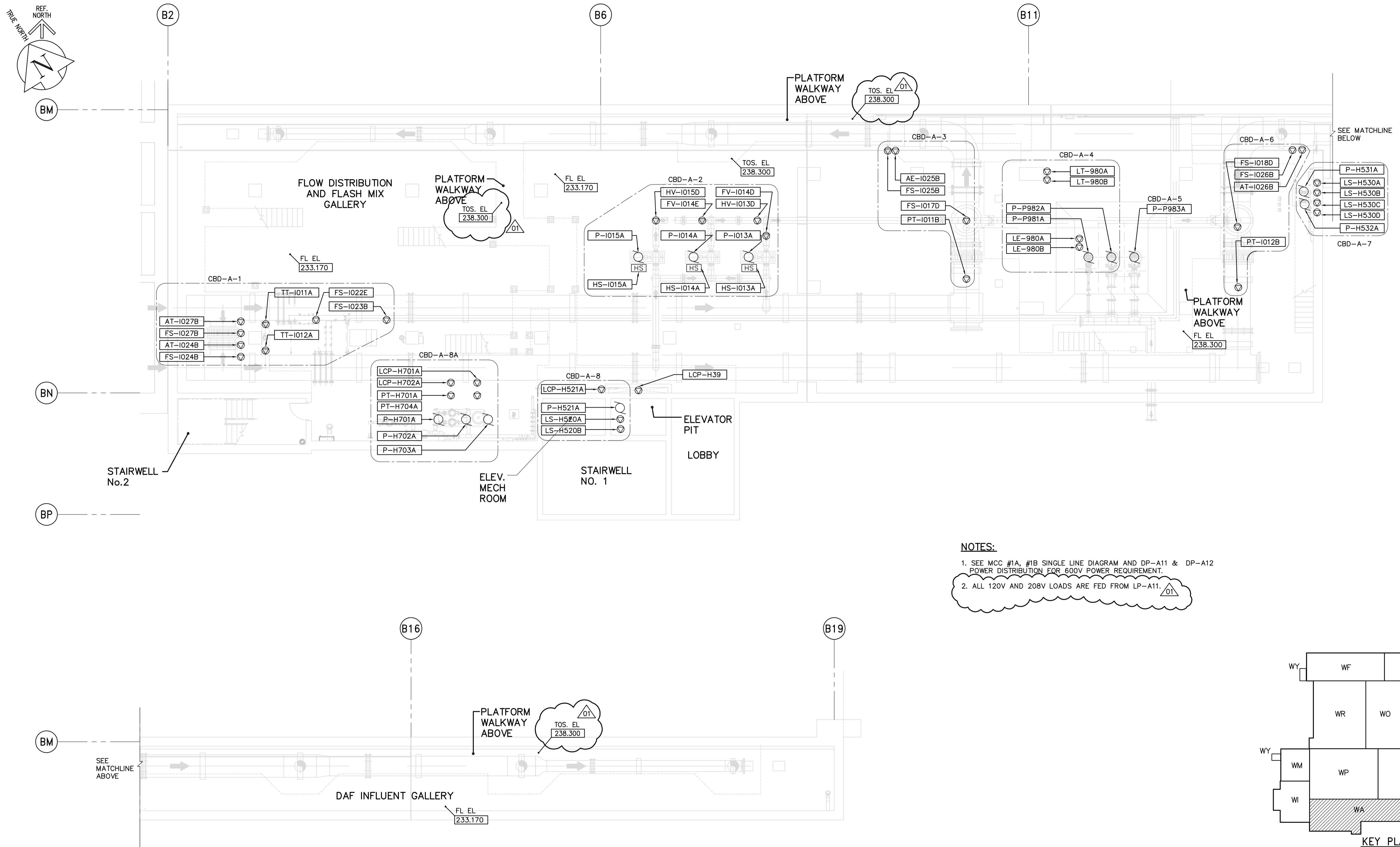
LOWER LEVEL PROCESS PLAN 1:100
