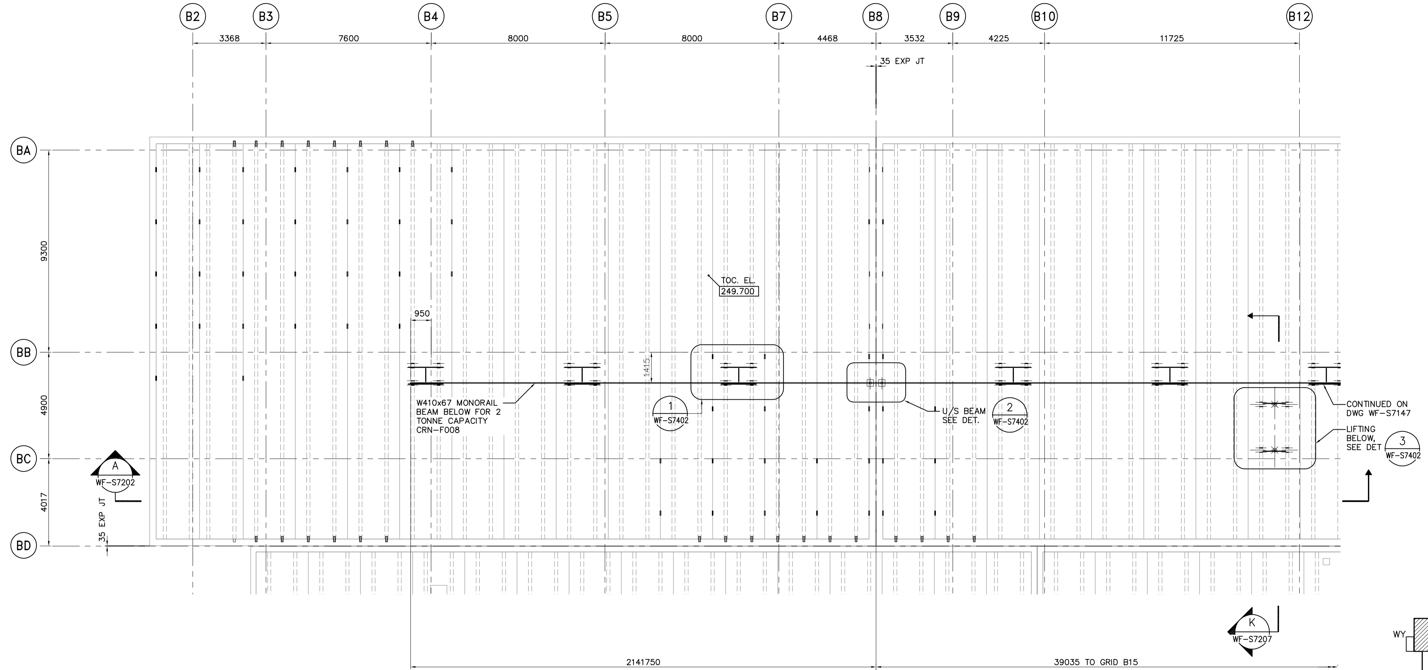
ROOF PLAN 1:100
