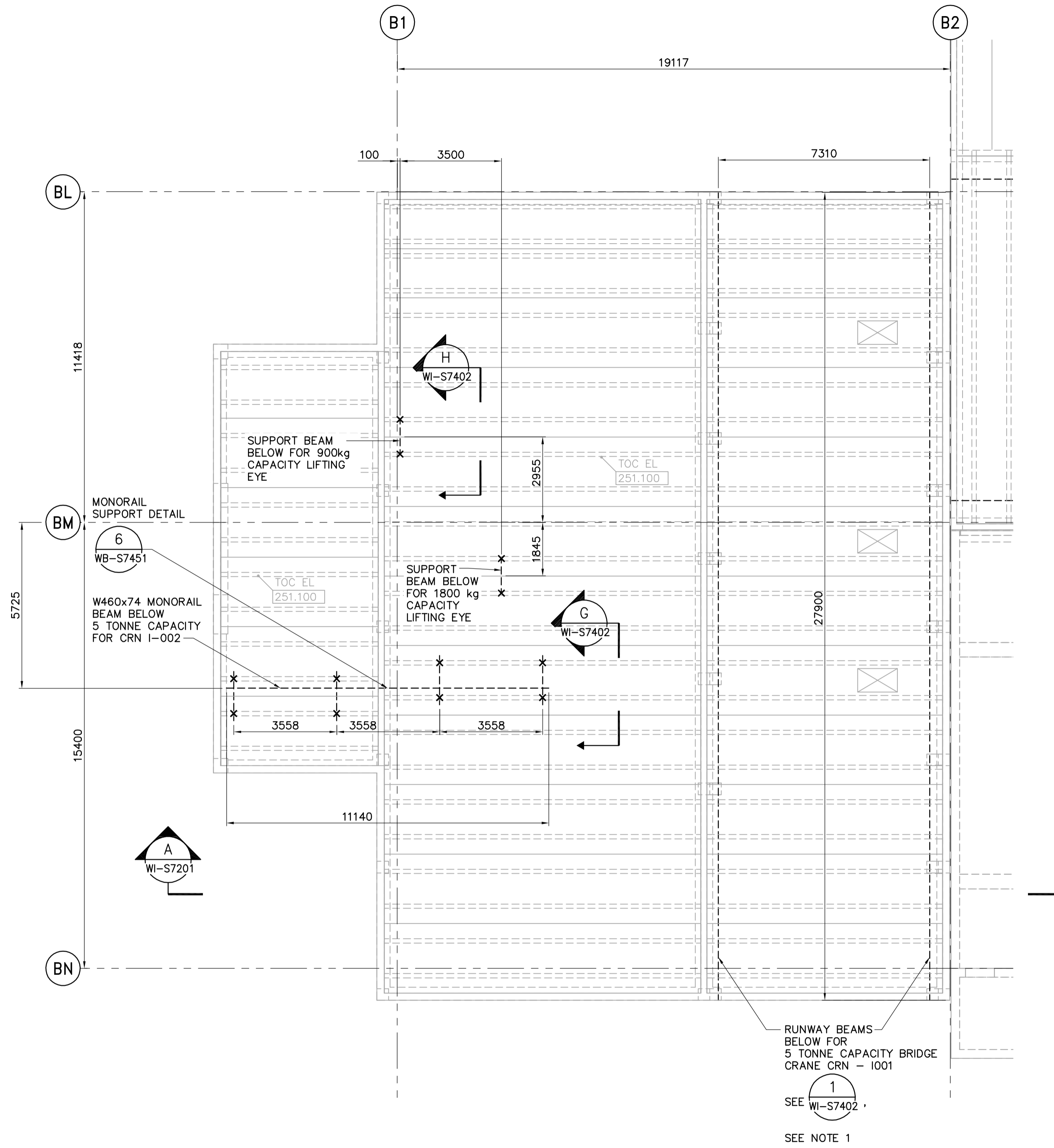
ROOF PLAN 1:100
