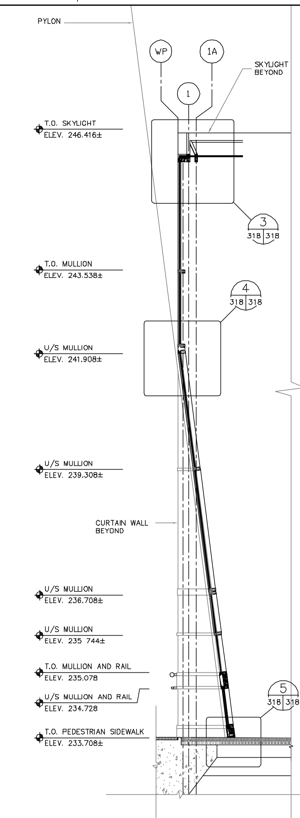
2 WALL SECTION @ GLAZING 316/318 1:30
