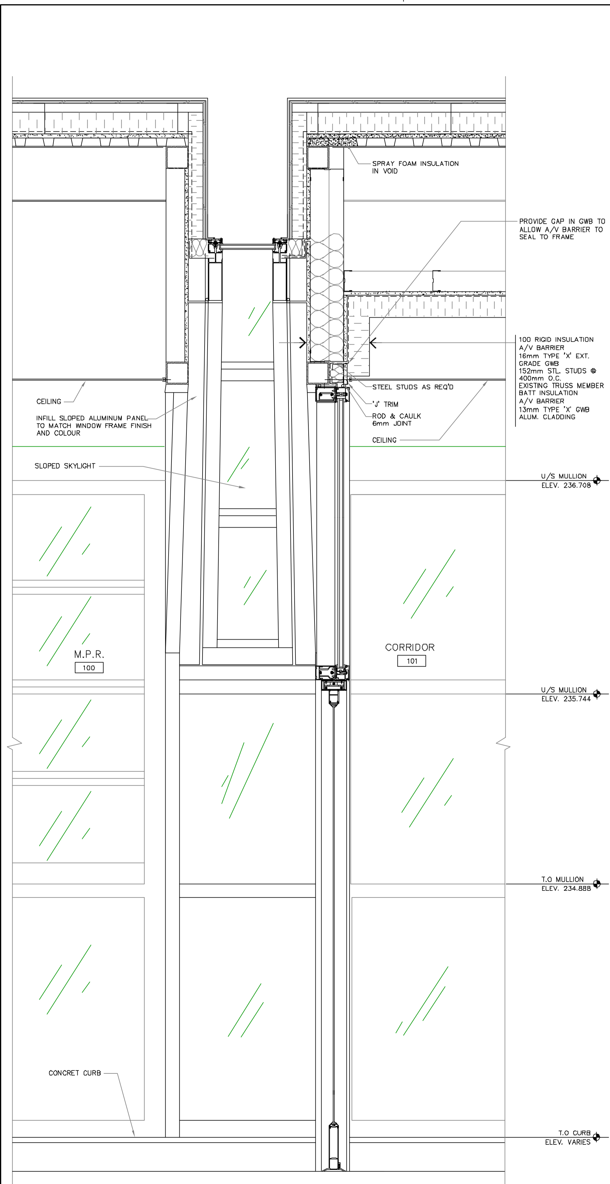
1 SECTION/ELEVATION - @ INTERIOR OF SKYLIGHT 316/318 1:20
