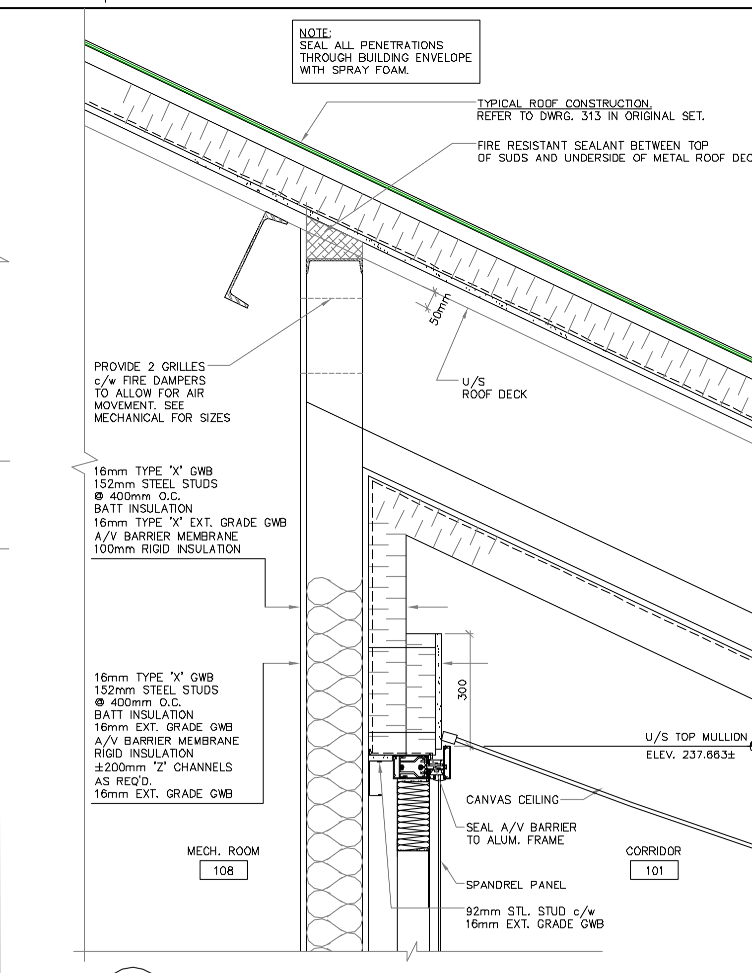
6 SECTION DETAIL 317/318 1:10
