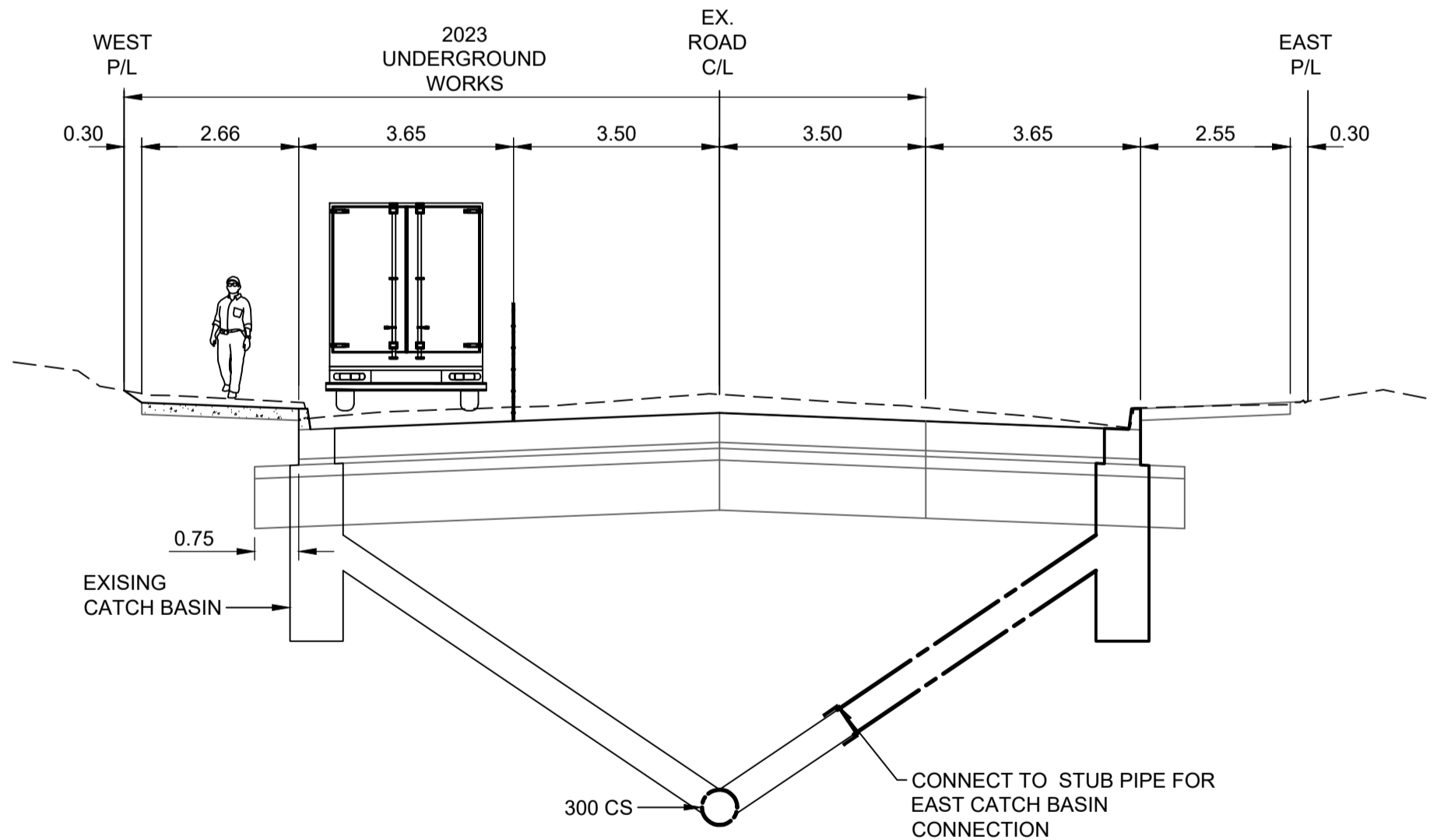
2023 STAFFORD UG WORKS NORTH OF HECTOR SCALE 1:100
