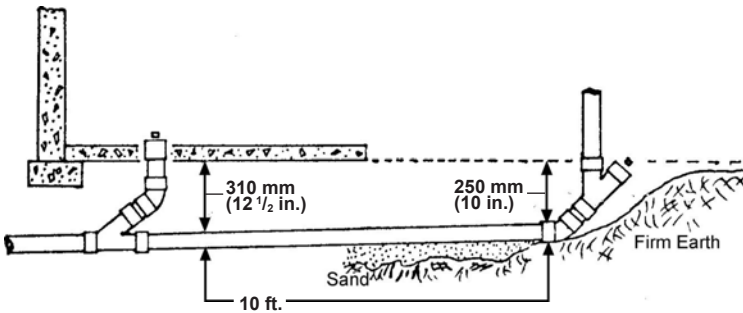
FIGURE 2 - Minimum Slope of Drains
