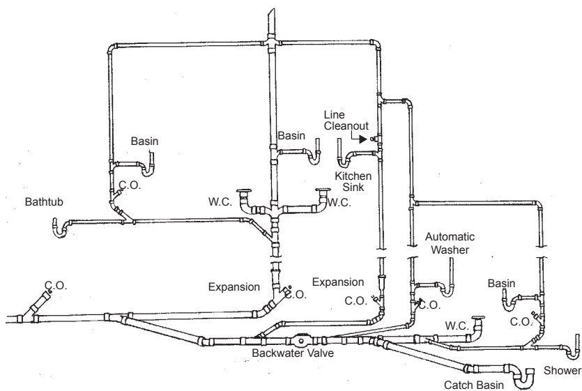
FIGURE 5 - Building Drainage System With Cleanout Fittings
