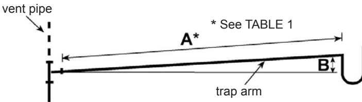
FIGURE 3 - Fall of Fixture Trap
