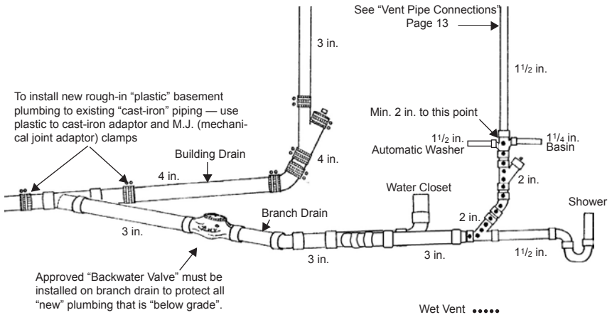
FIGURE 11 - Typical Basement Plumbing Installation Showing Venting Method, Backwater Valve & Attachment to "Cast-Iron" Piping
