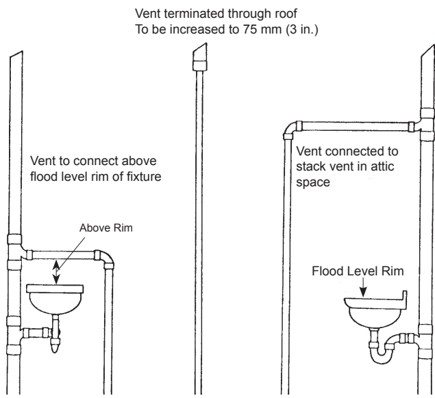
FIGURE 13 - Vent Pipe Connections
