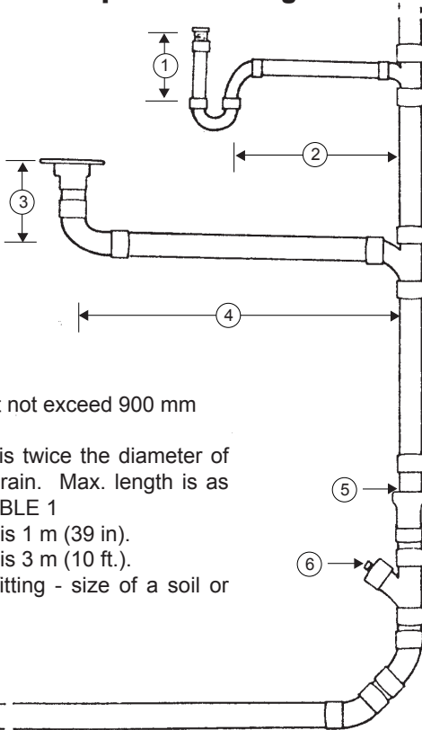
FIGURE 4 - Lengths of Fixture Drains and Expansion Fitting
