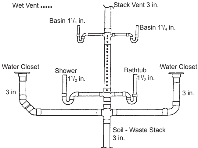
FIGURE 9 - One Storey Venting (Back to Back)
