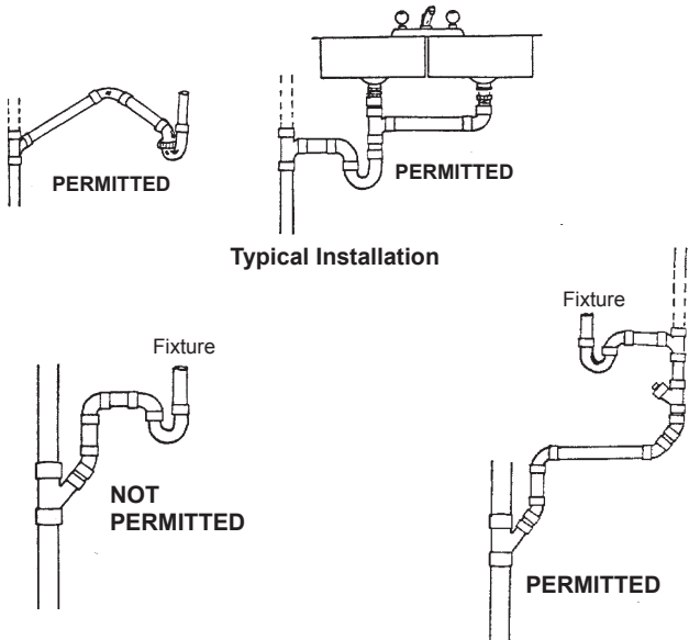
FIGURE 8 - Permitted Use of Sanitary "T" ("TY") Fittings - Exceptions
