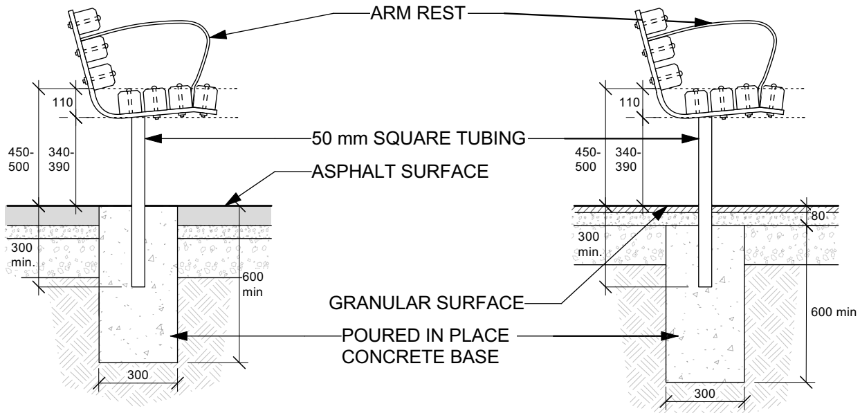
SIDE ELEVATION - ASPHALT
