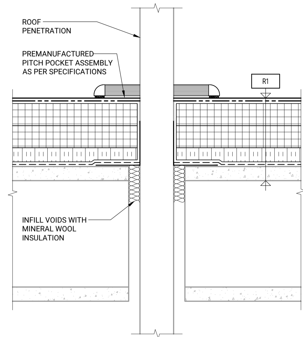
4 TYPICAL PITCH POCKET DETAIL
