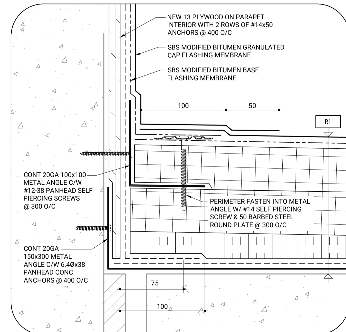
A TYPICAL PERIMETER FASTENING DETAIL
