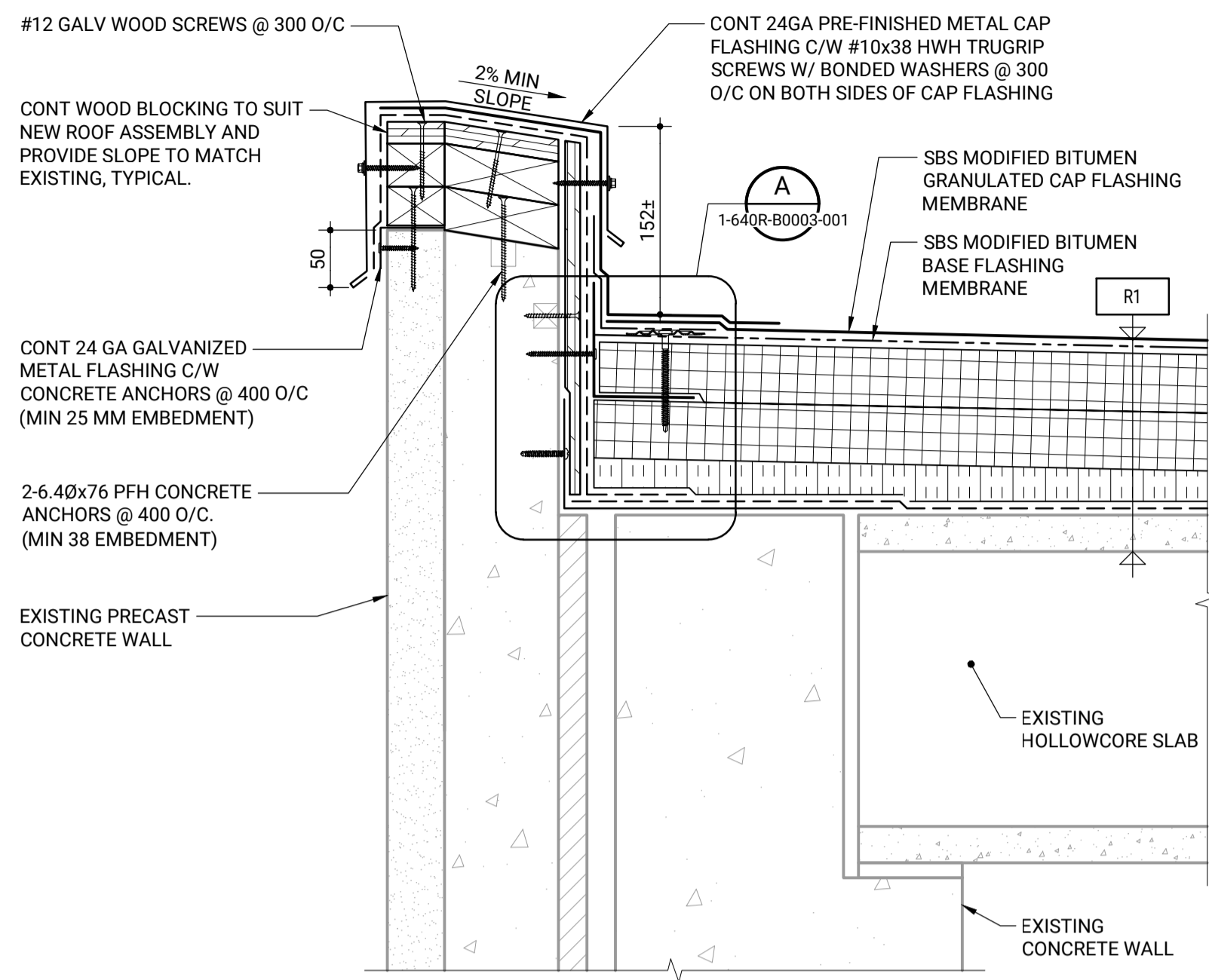
1 TYPICAL ROOF PARAPET DETAIL
