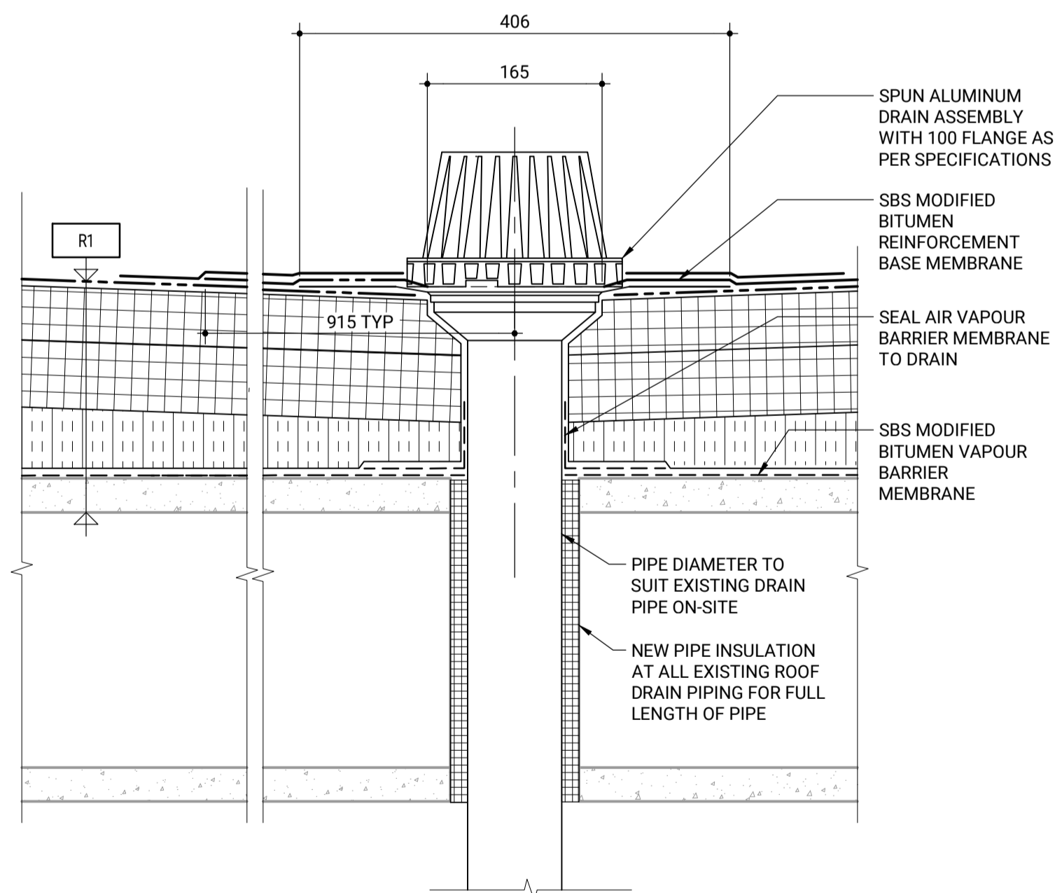
6 TYPICAL DRAIN DETAIL
