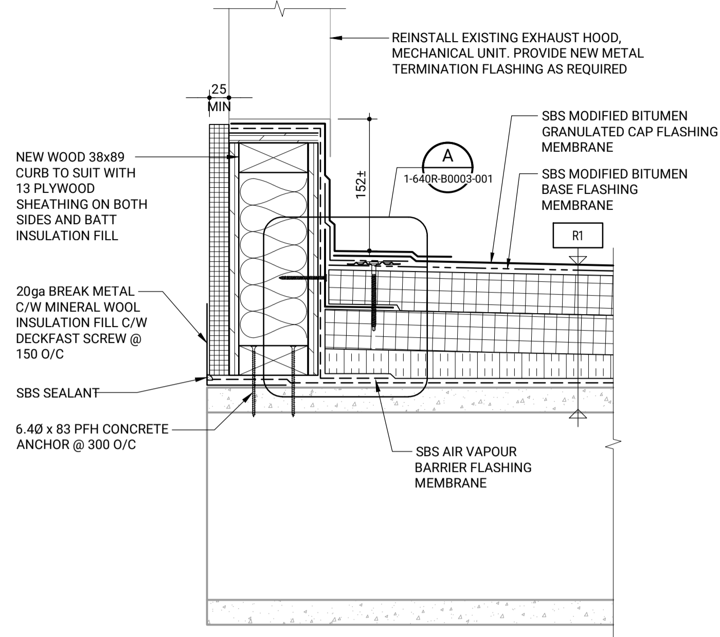
3 TYPICAL CURB DETAIL
