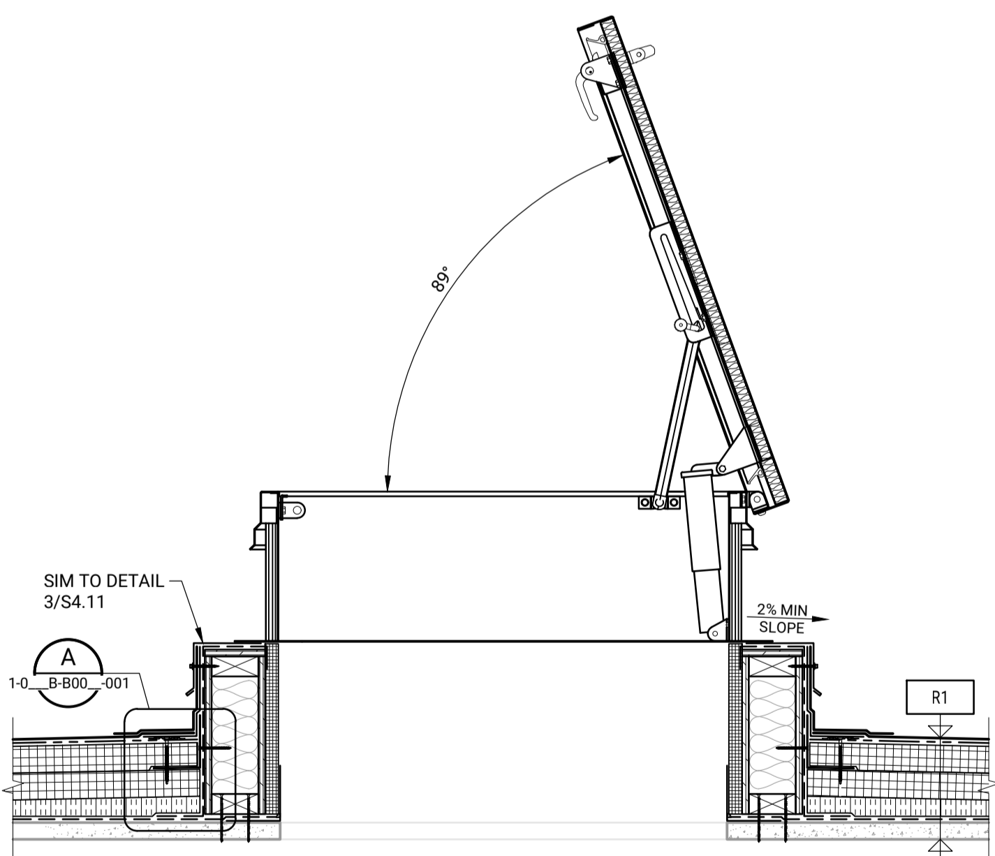
5 ROOF HATCH DETAIL
