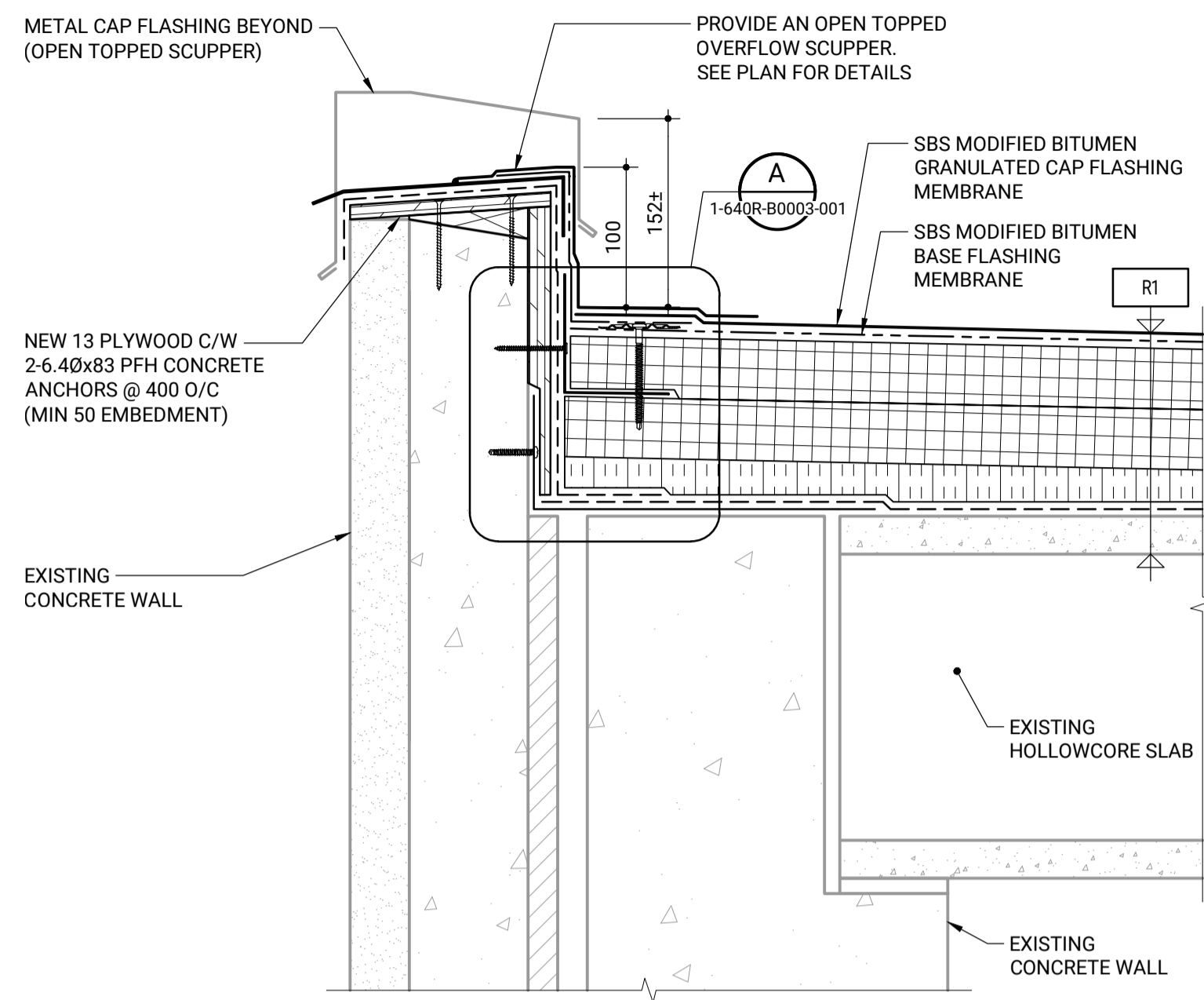
2 TYPICAL OVERFLOW SCUPPER DETAIL
