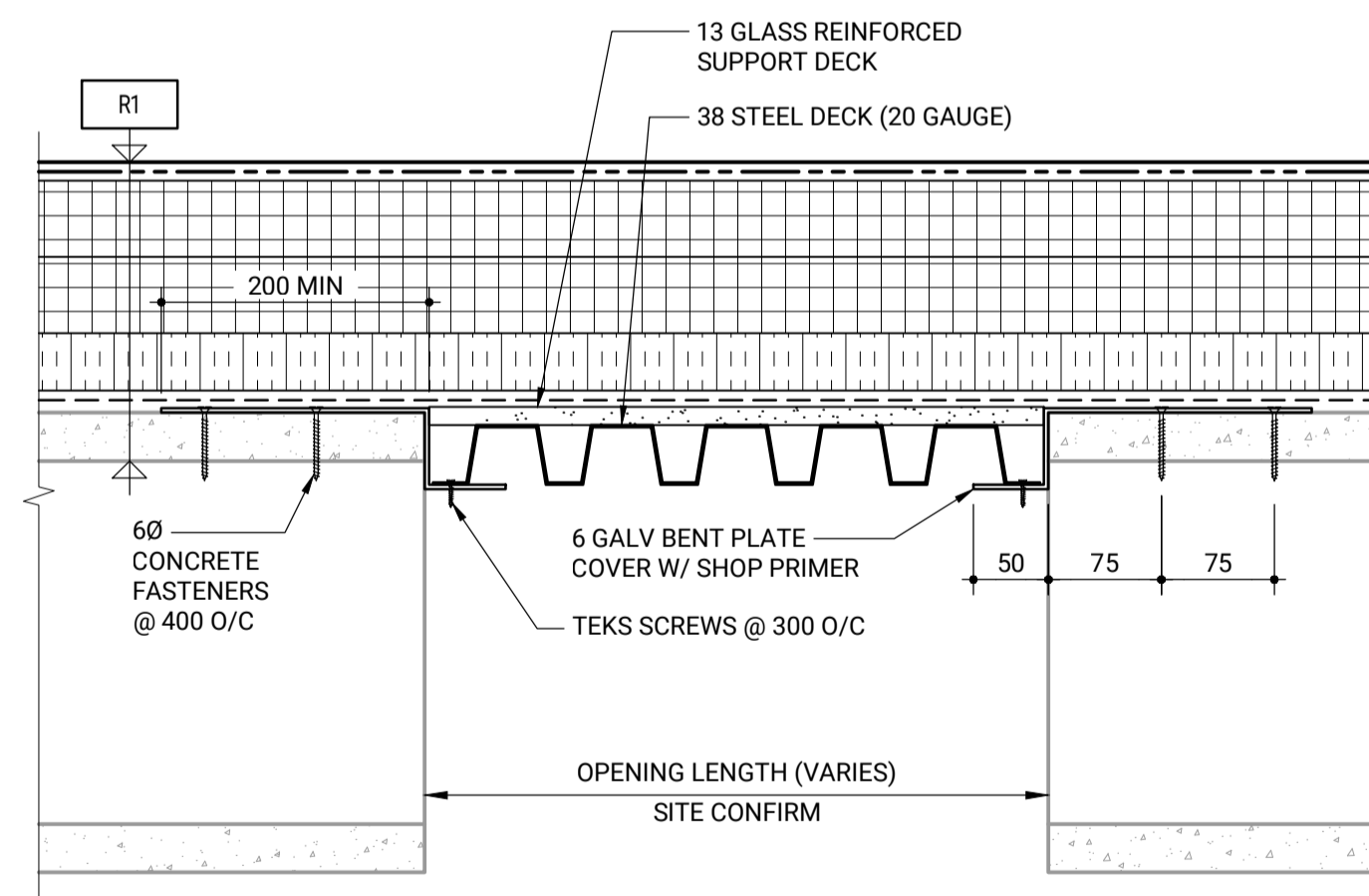
7 TYPICAL CONCRETE DECK INFILL DETAIL
