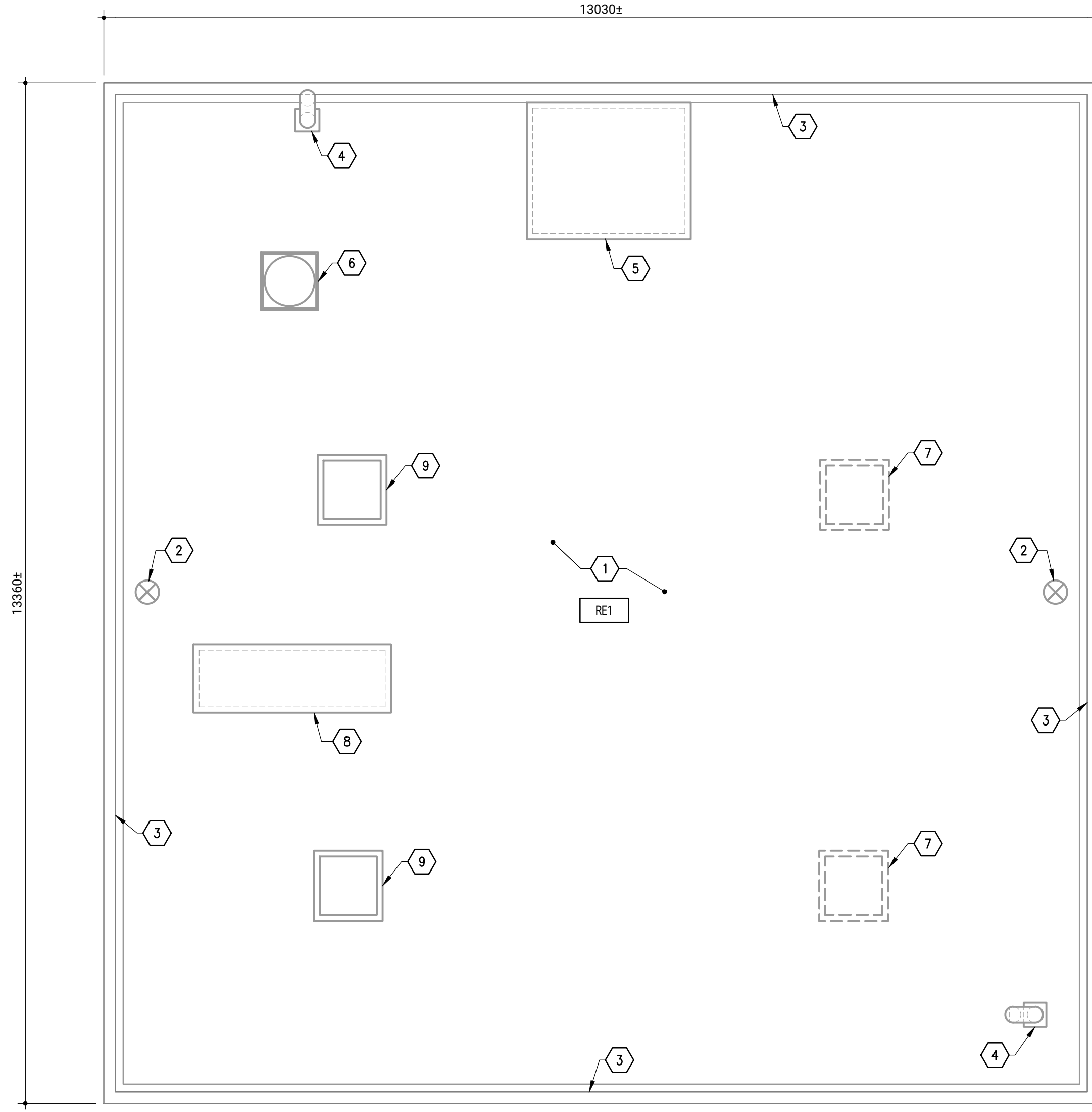
ROOF PLAN - DEMOLITION 1:50
