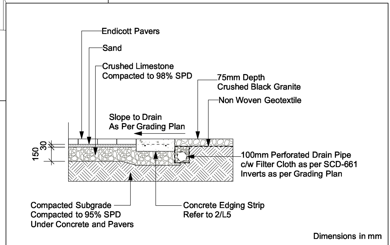
2 DRAIN PIPE ALONG CONCRETE EDGE L4 1:25
