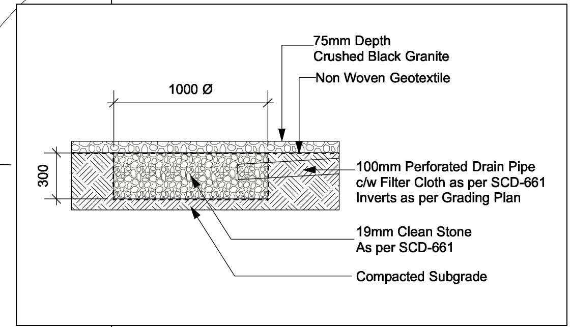
3 SUMP PIT L4 1:25
