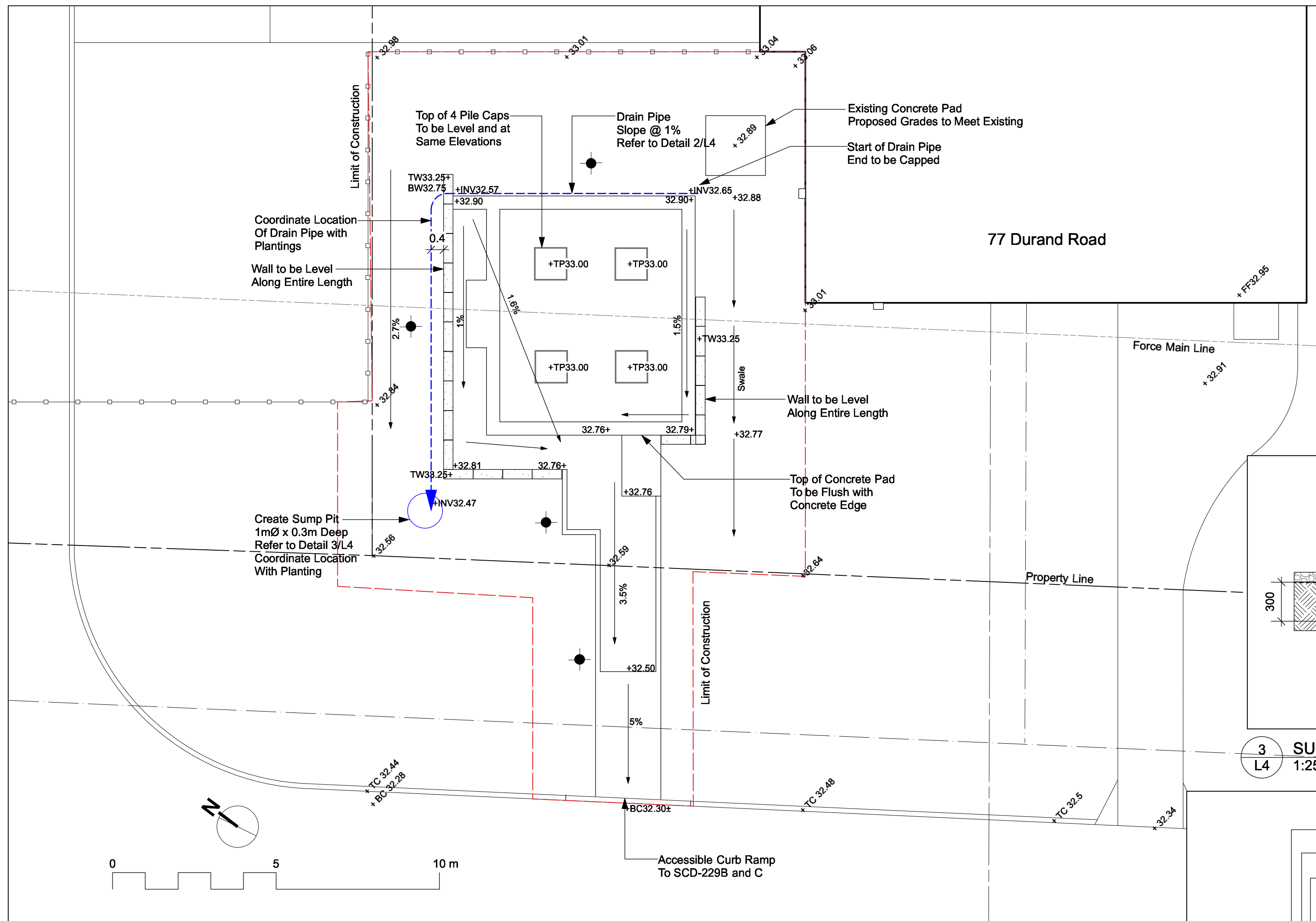
1 GRADING PLAN L4 1:100
