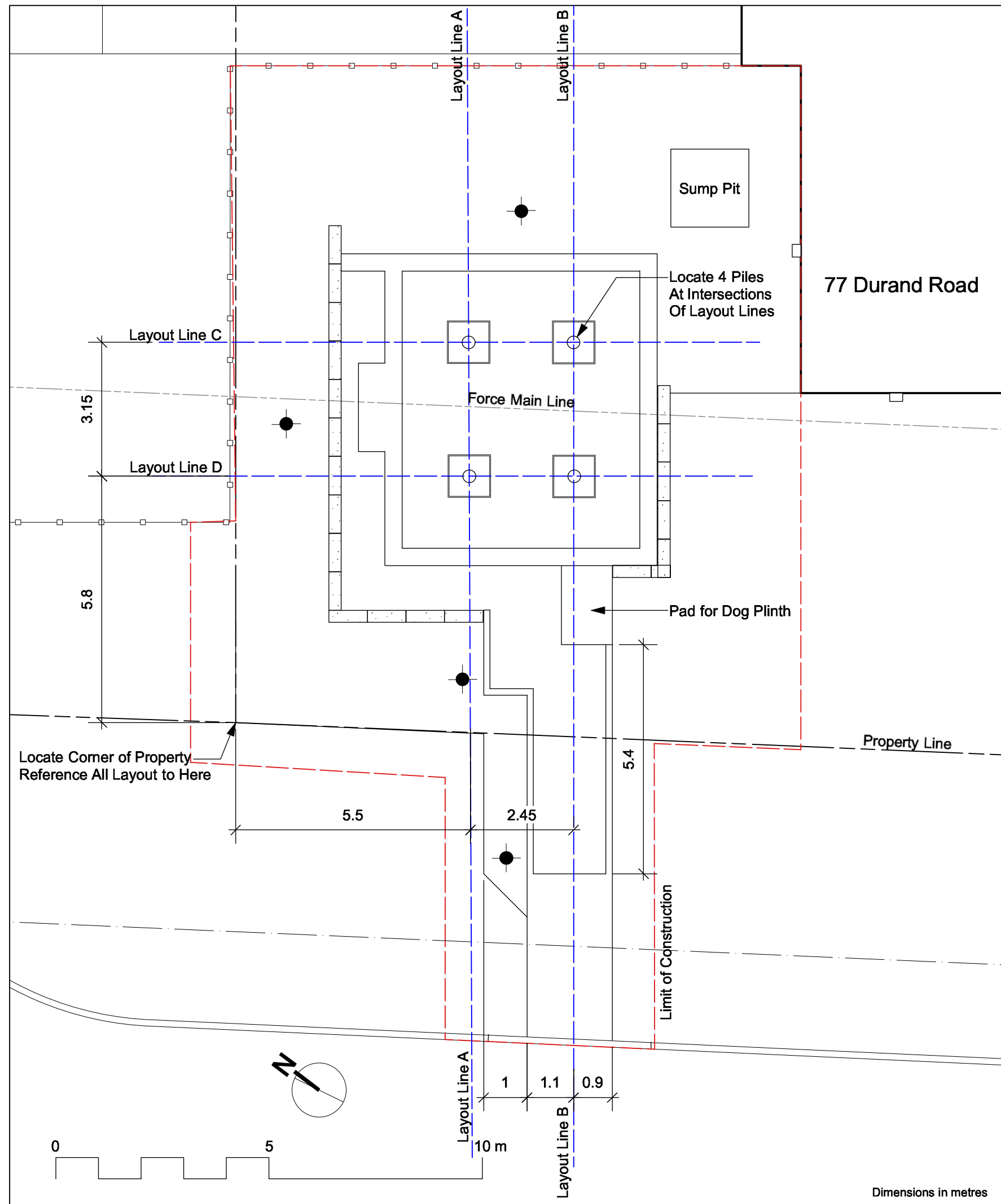
1 L3 GENERAL LAYOUT 1:100
