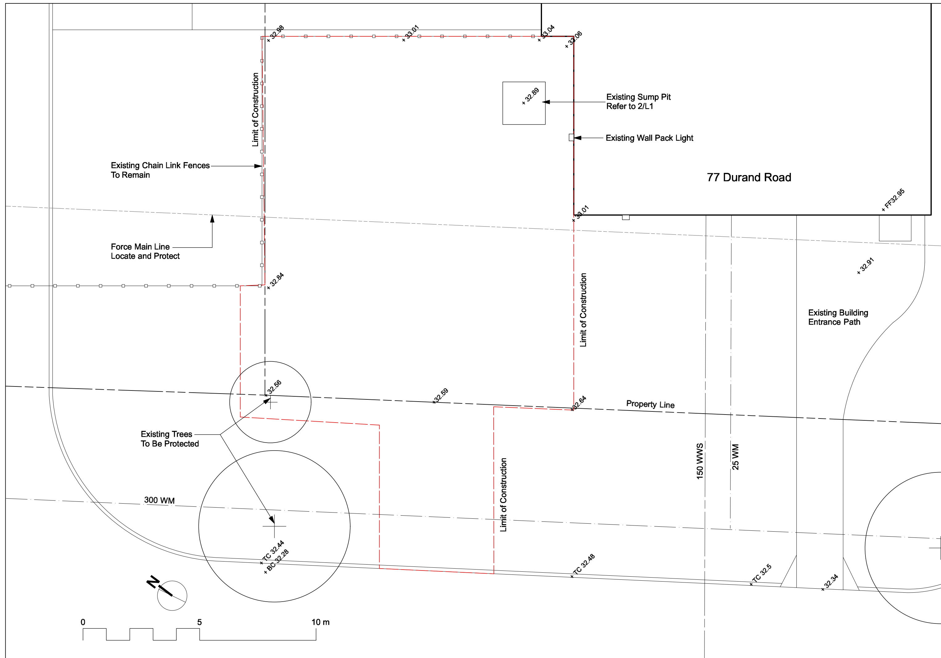
1 EXISTING CONDITIONS L1 1:100
