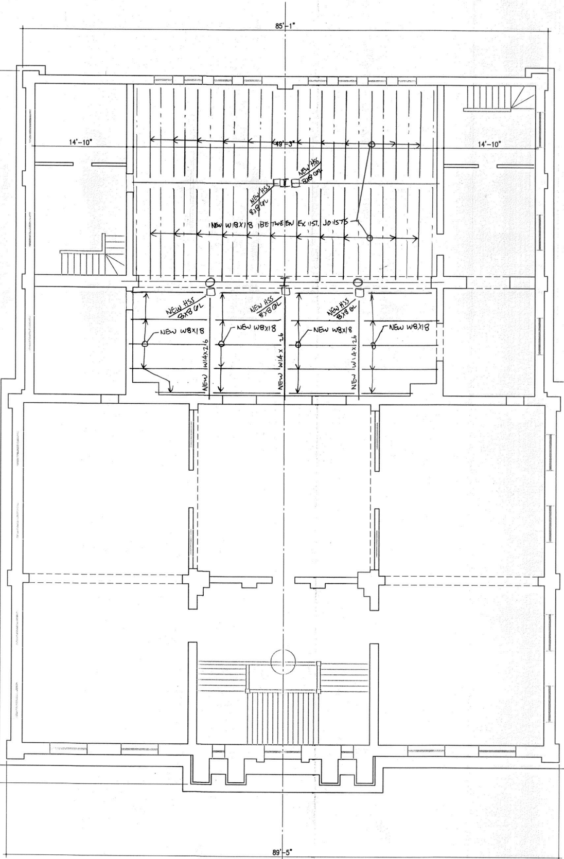
SECOND MEZZANINE PLAN
