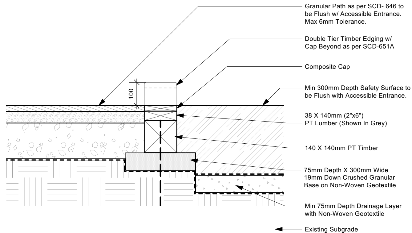
1 C.65 - G Accessible Entrance Scale: 1:10
