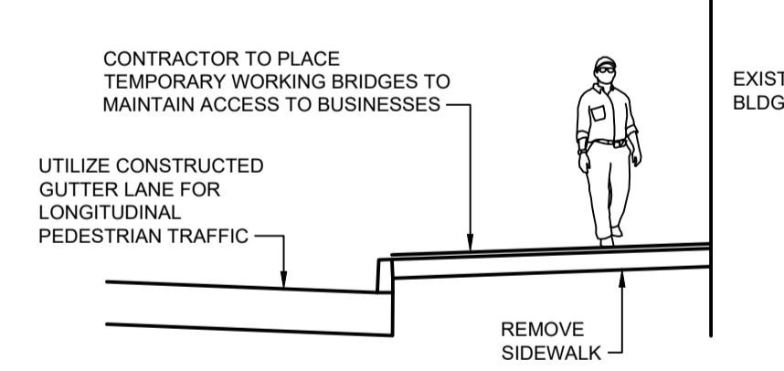
PEDESTRIAN ACCESS DURING SIDEWALK CONSTRUCTION SCALE N.T.S.
