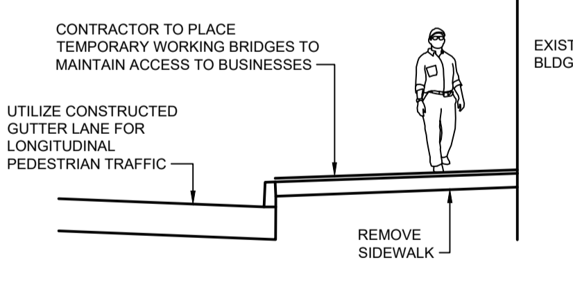
PEDESTRIAN ACCESS DURING SIDEWALK CONSTRUCTION SCALE N.T.S.
