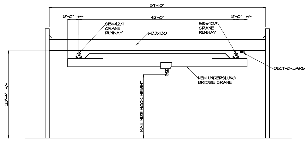
SECTION
