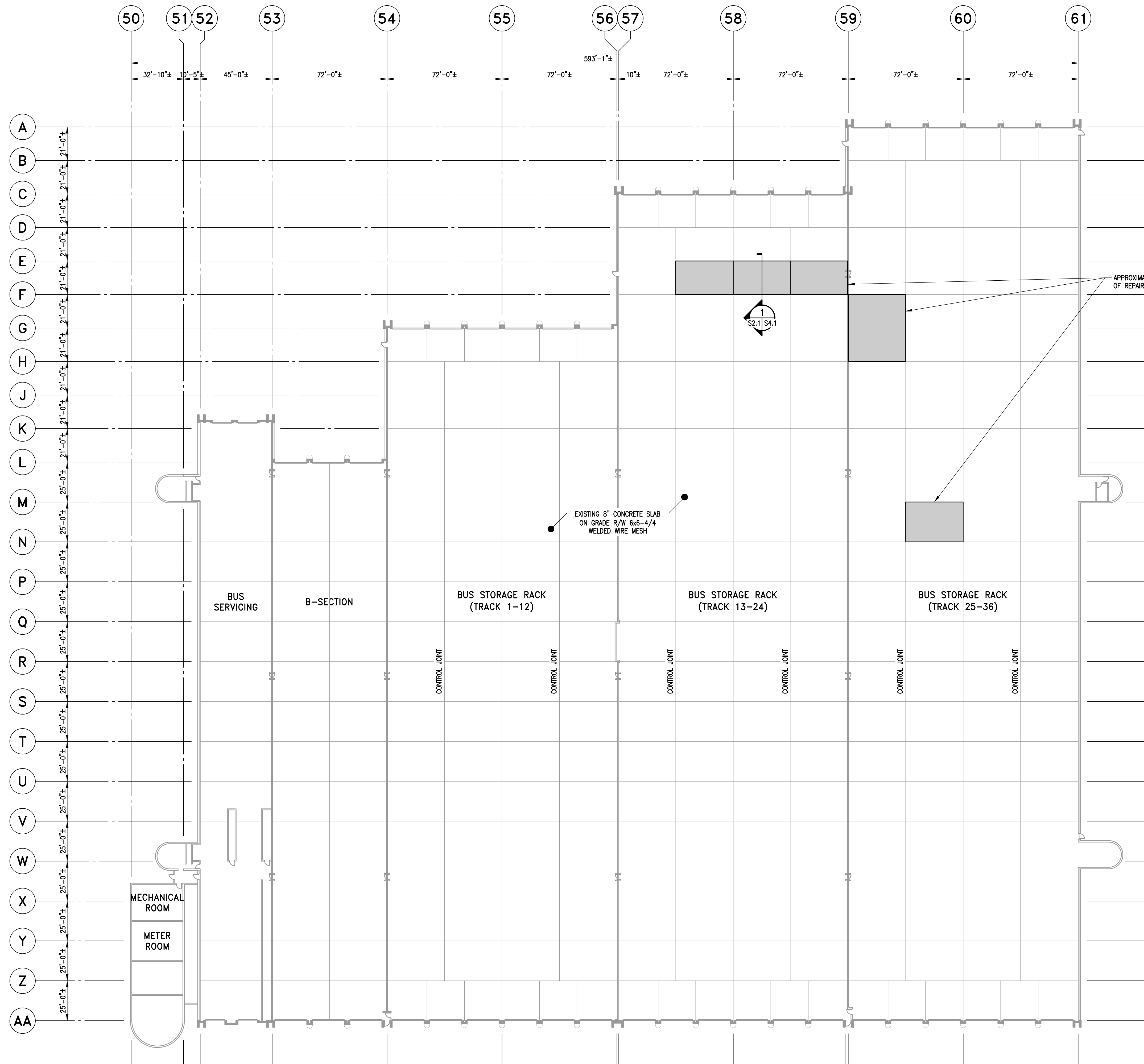
MAIN FLOOR PLAN 1/32" = 1'-0"
