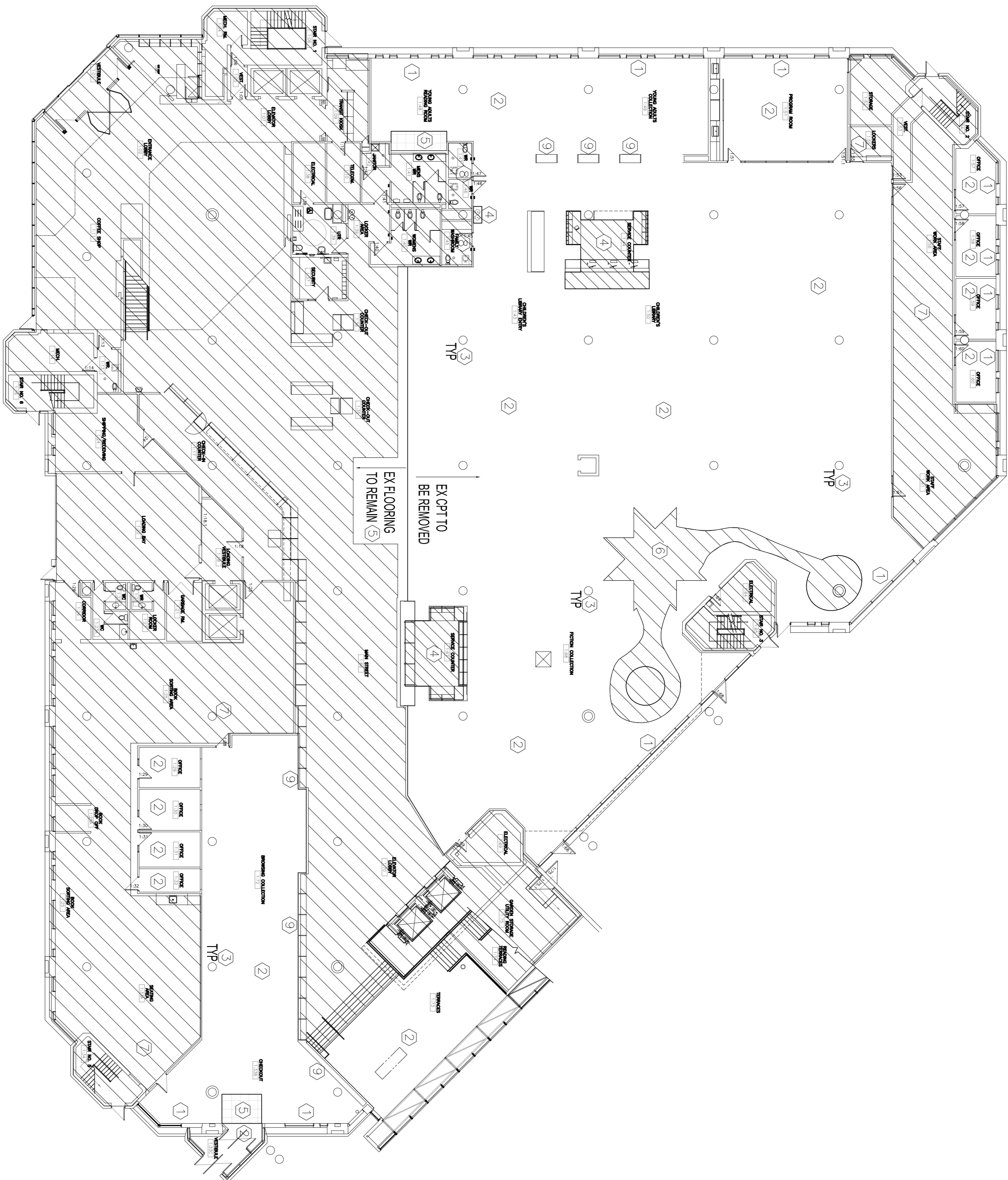
1 MAIN FLOOR - DEMOLITION PLAN A1.1 SCALE: 1/8"=1'-0"
