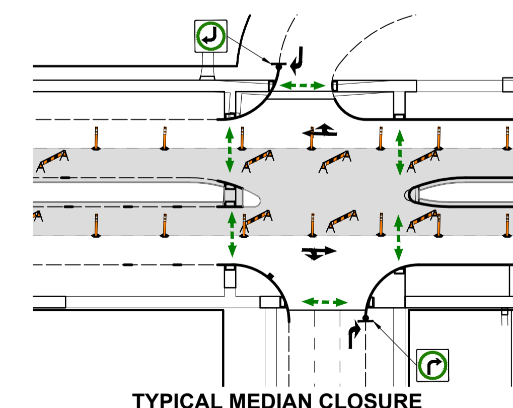
TYPICAL MEDIAN CLOSURE
