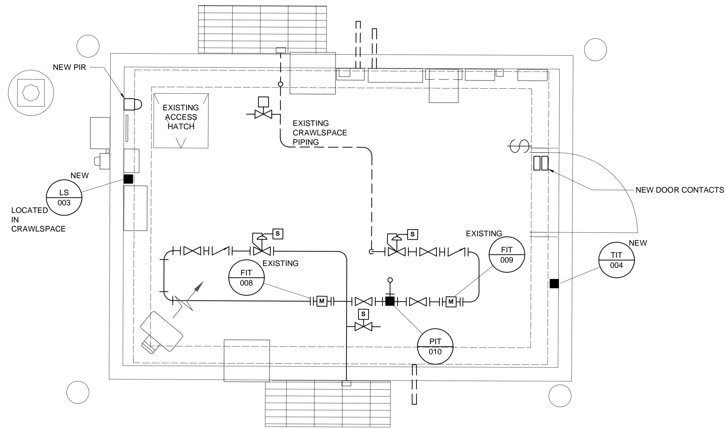
NEW BUILDING INSTRUMENTATION PLAN SCALE 1:25
