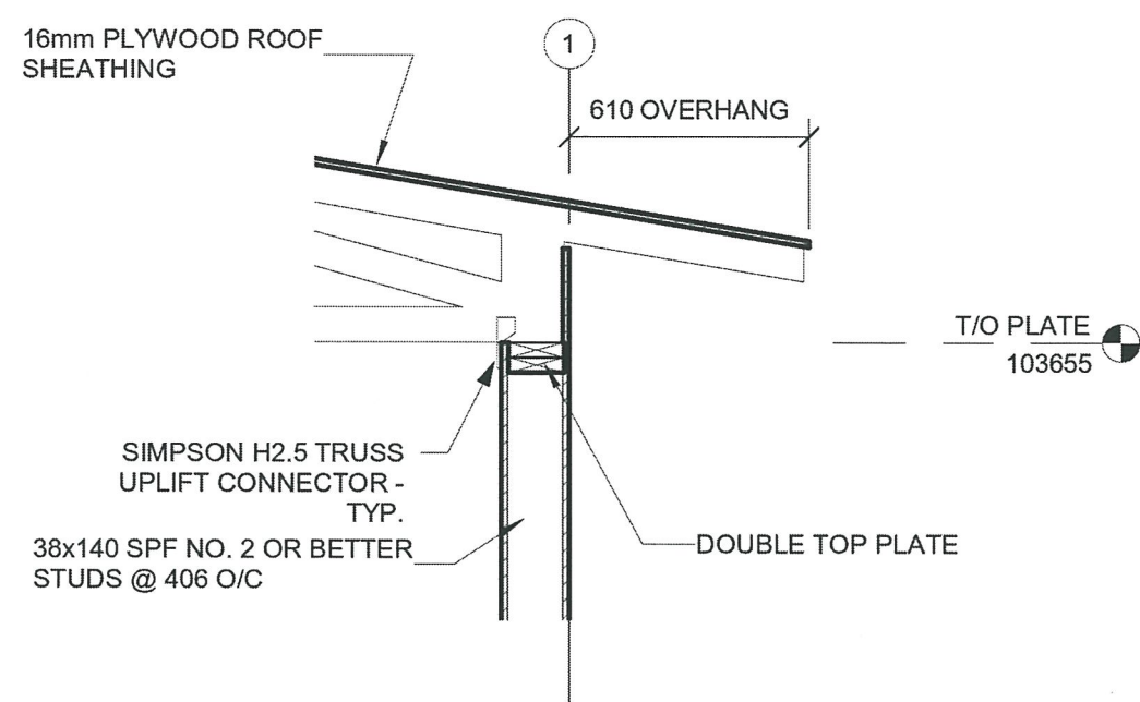
2 SECTION S501 1:20
