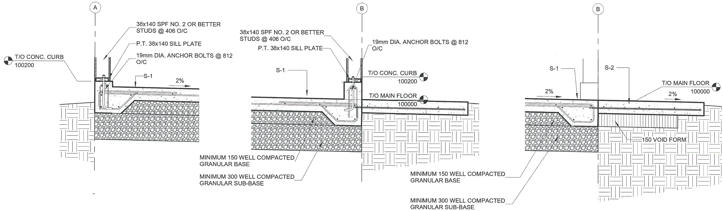
1 WALL SECTION S401 1:20
