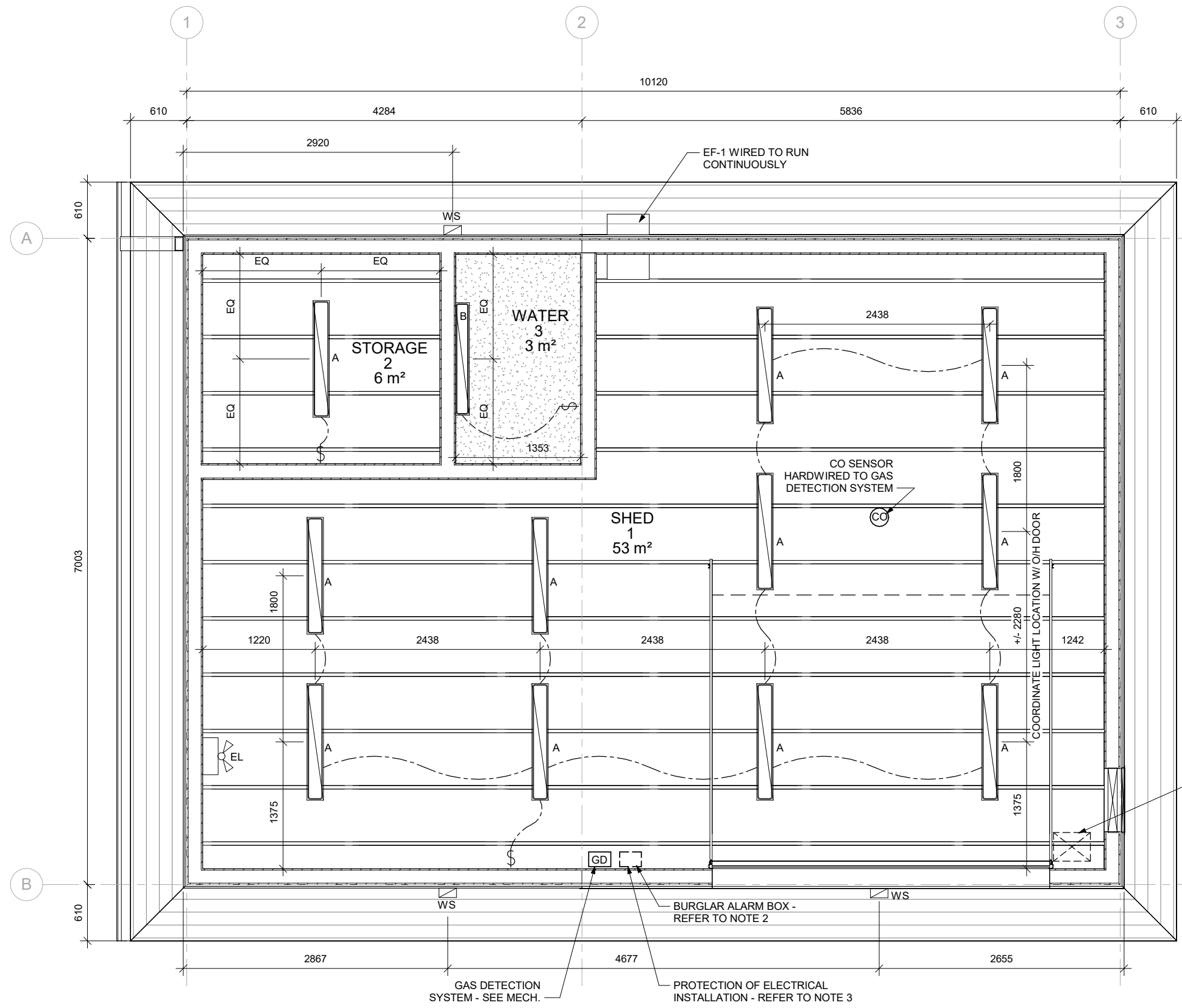
1 E - REFLECTED CEILING PLAN 1:50
