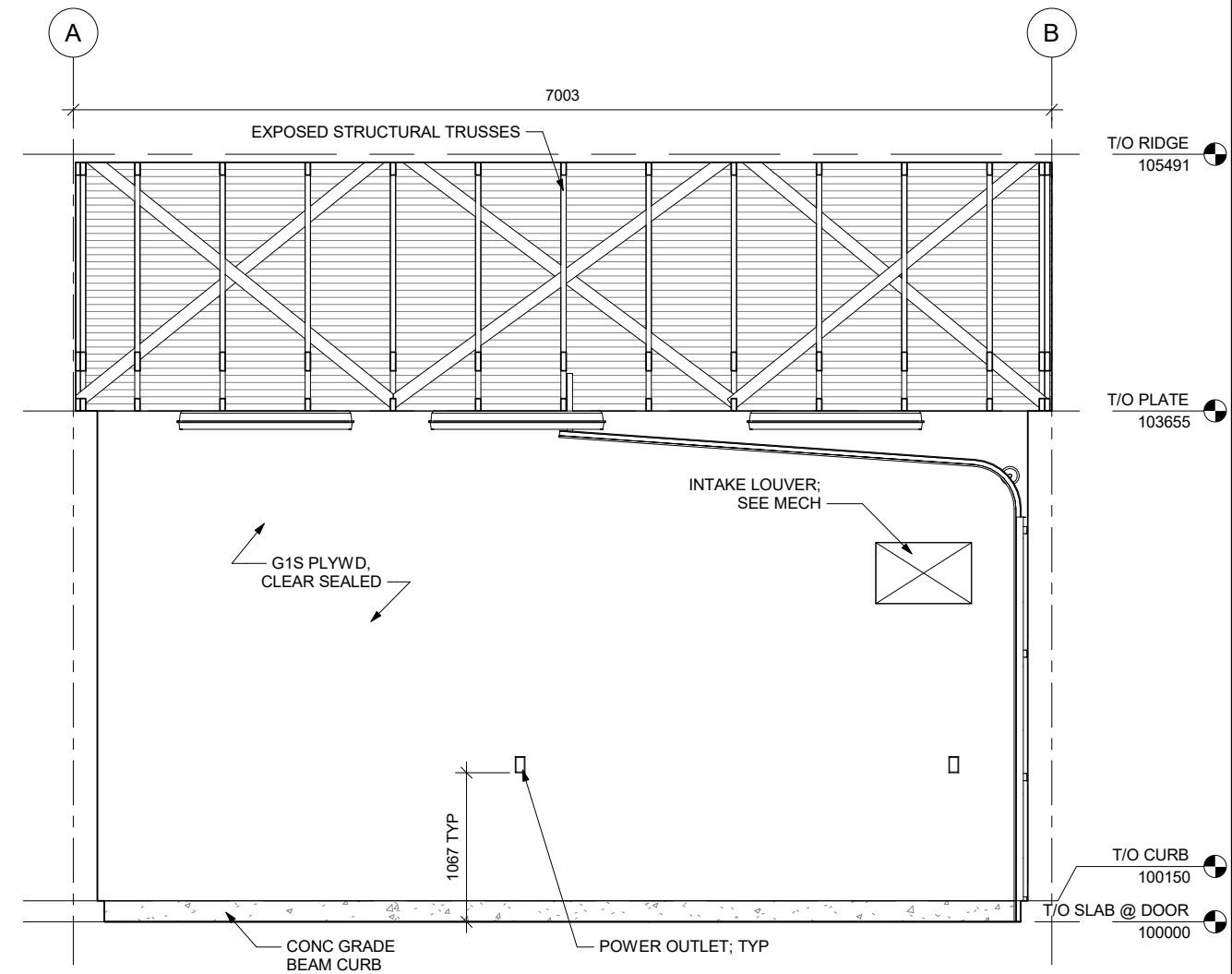
2 INT ELEVATION - GARAGE - B 1:50
