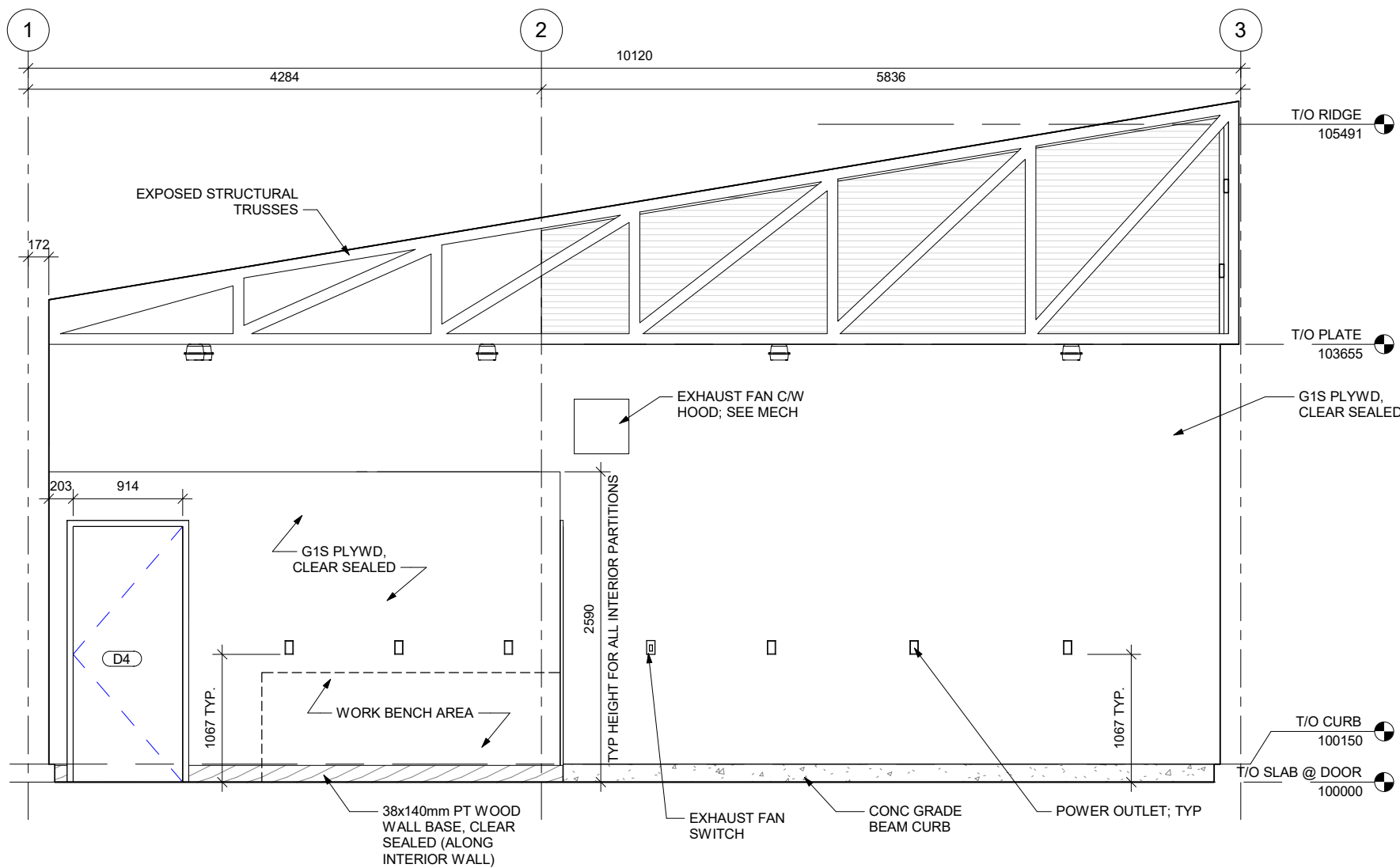
1 INT ELEVATION - GARAGE - A 1:50
