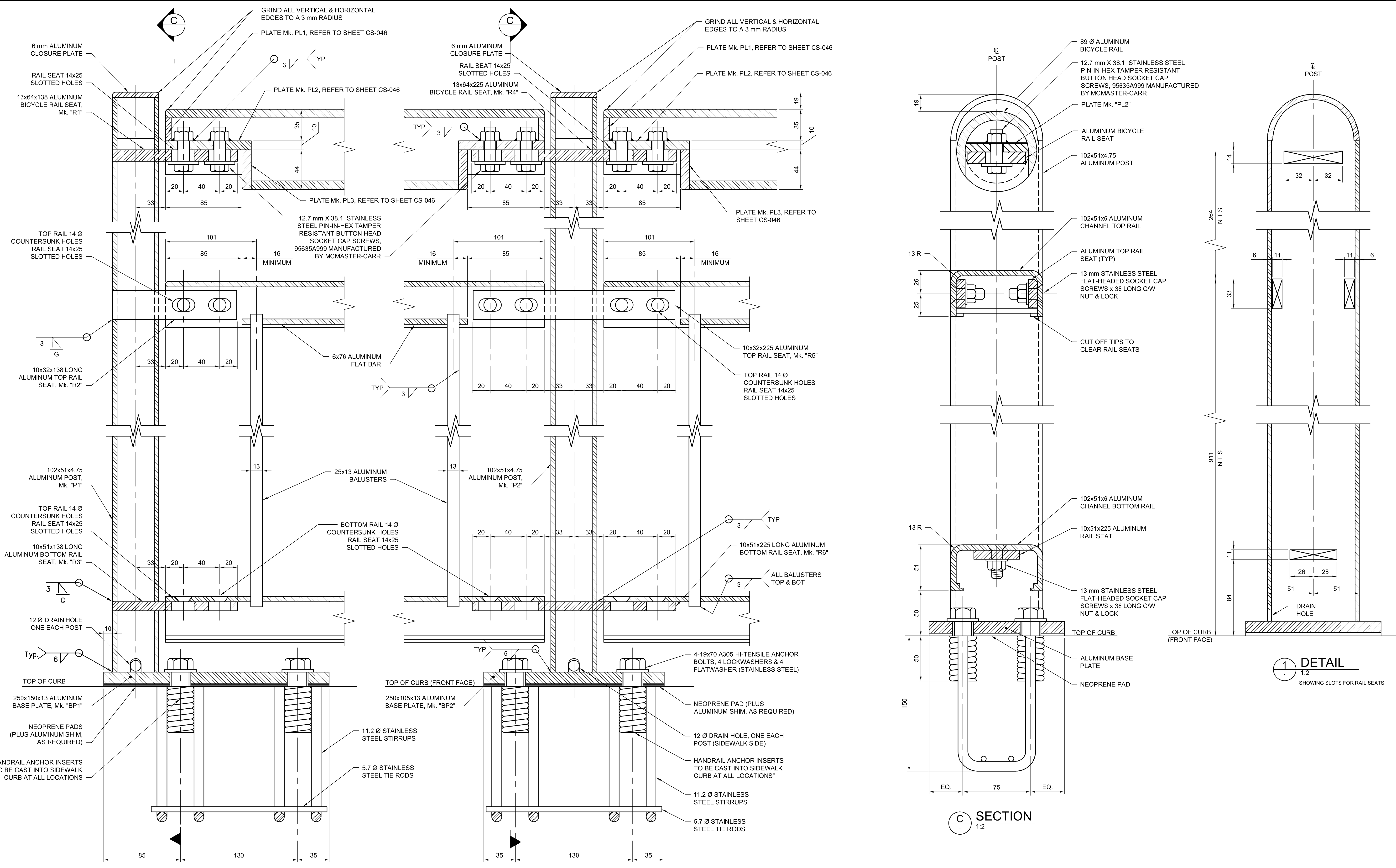
DETAIL AT END POSTS Mk. "P1" 1:2
