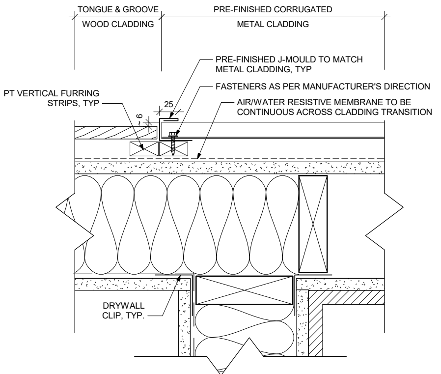
5 PLAN DETAIL - TYPICAL WOOD TO MTL TRANSITION 1:5
