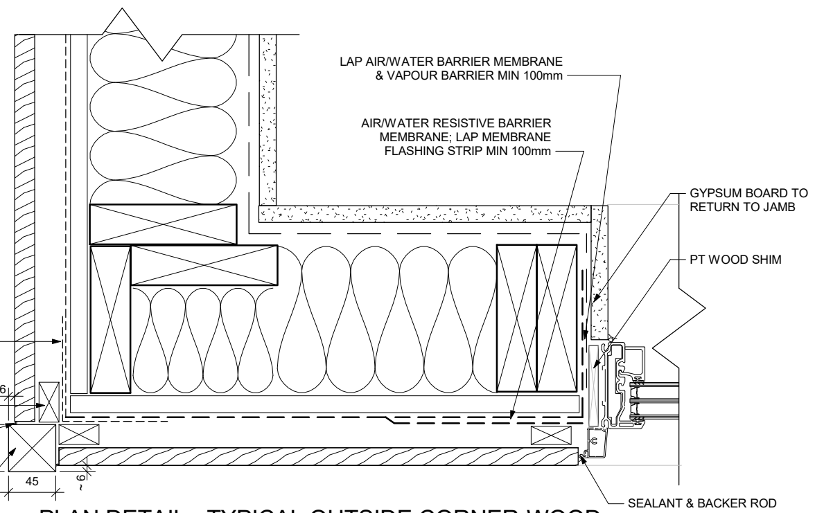
7 PLAN DETAIL - TYPICAL OUTSIDE CORNER-WOOD 1:5
