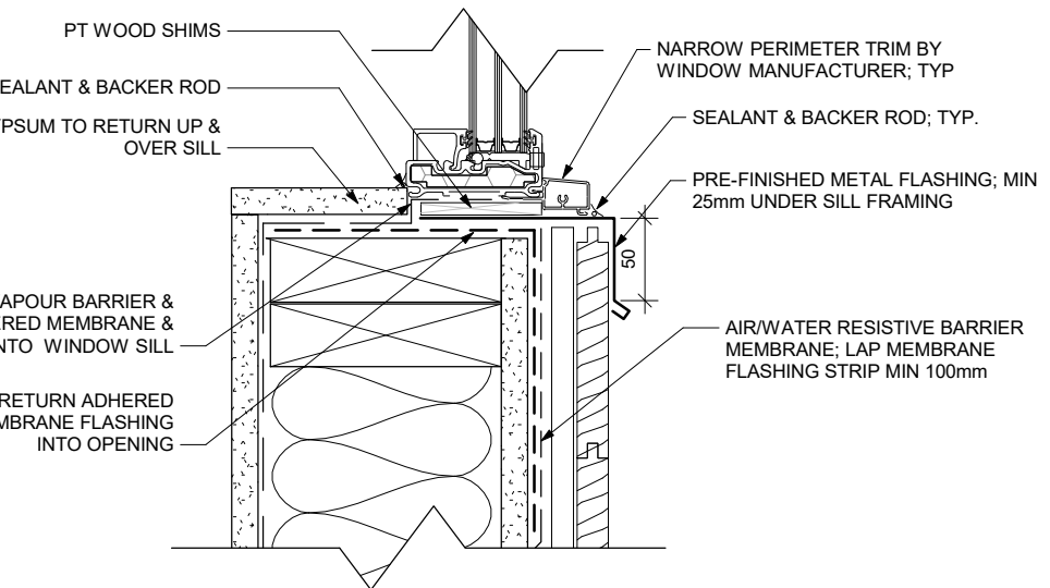
1 SECTION DETAIL - TYPICAL WINDOW 1:5
