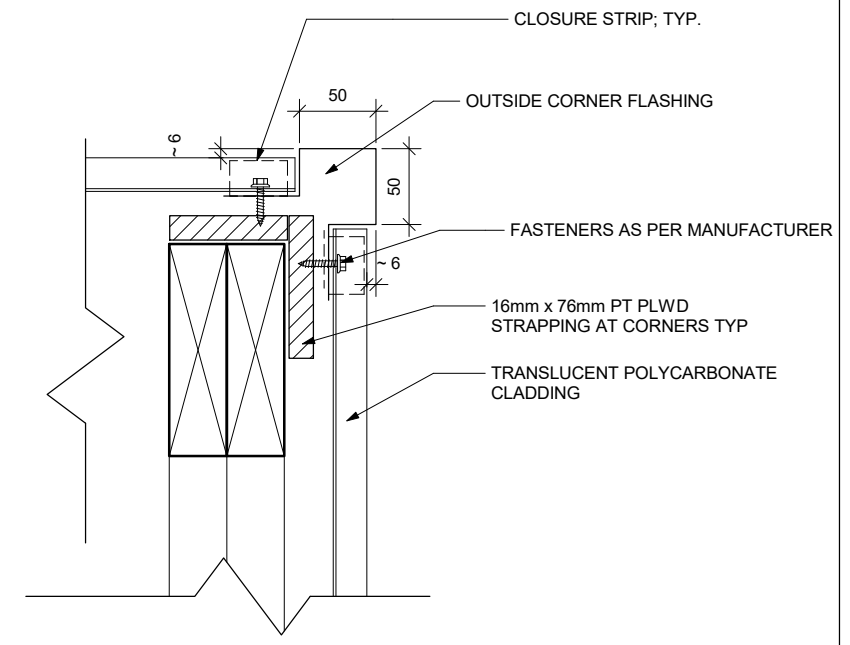
6 PLAN DETAIL - TYPICAL OUTSIDE CORNER-POLYCARB 1:5
