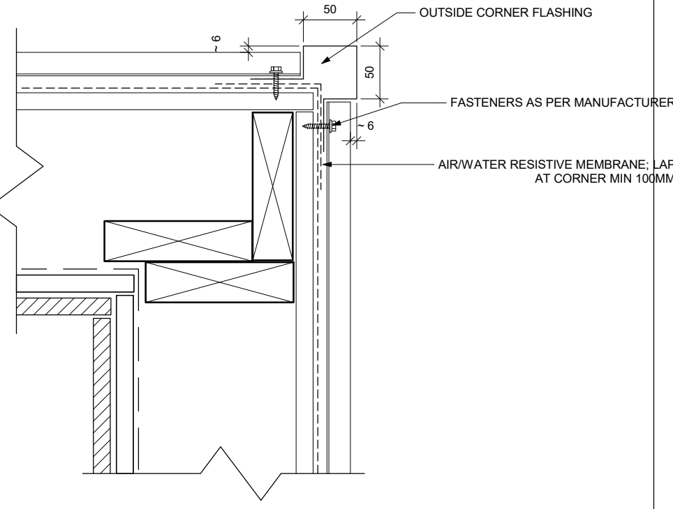
4 PLAN DETAIL - TYPICAL OUTSIDE CORNER 1:5
