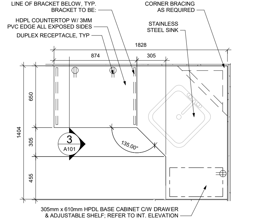
2 PLAN DETAIL - COUNTER 1 : 25
