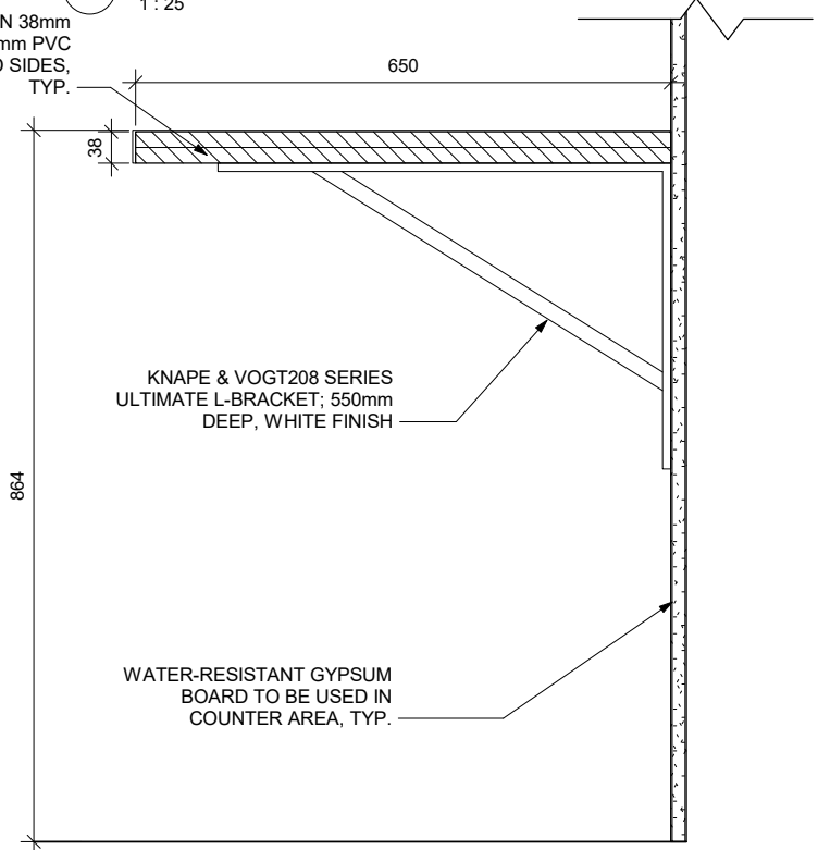
3 SECTION DETAIL - COUNTER 1 : 10
