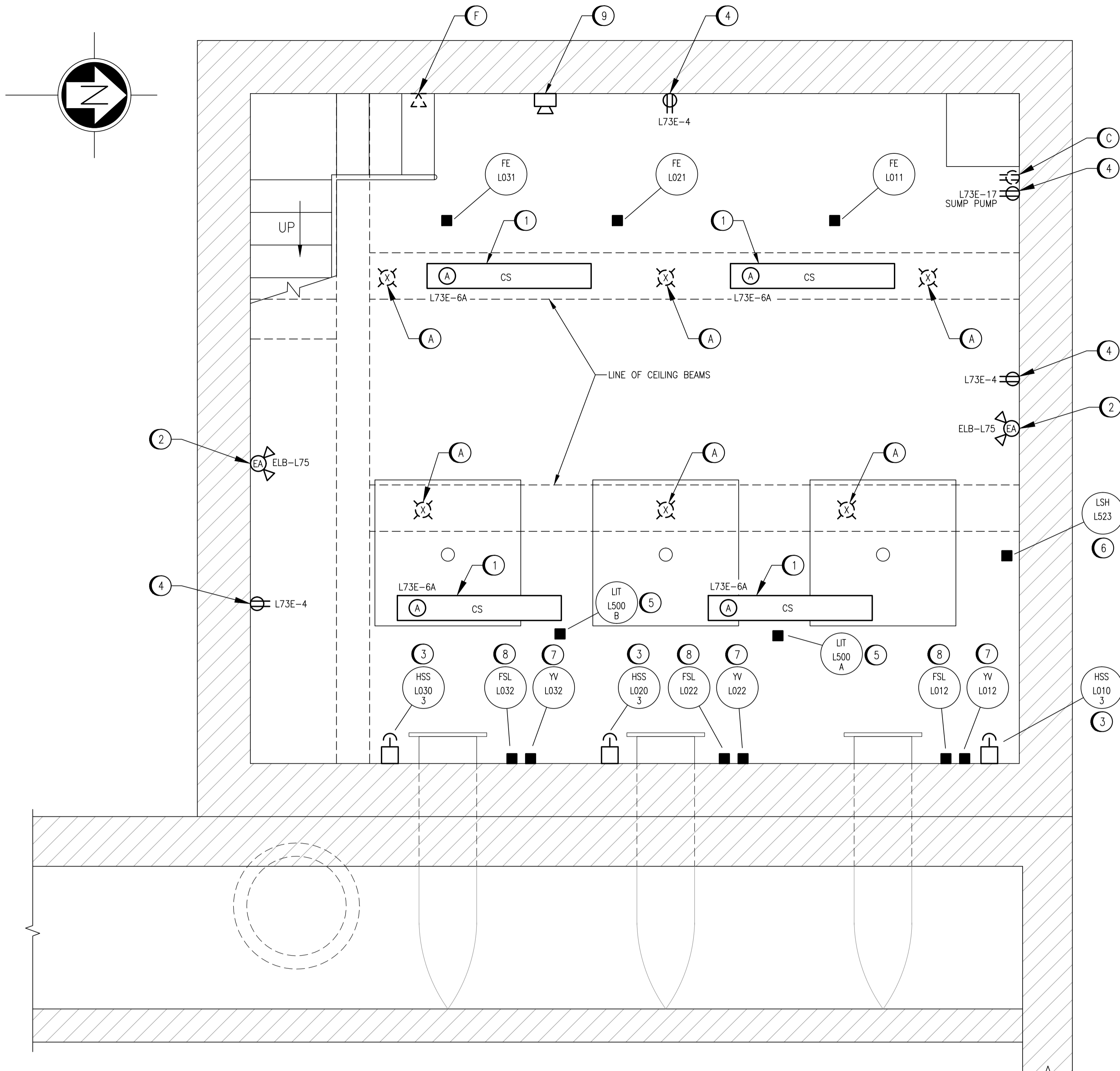
PUMP ROOM FLOOR PLAN SCALE: 1 : 20
