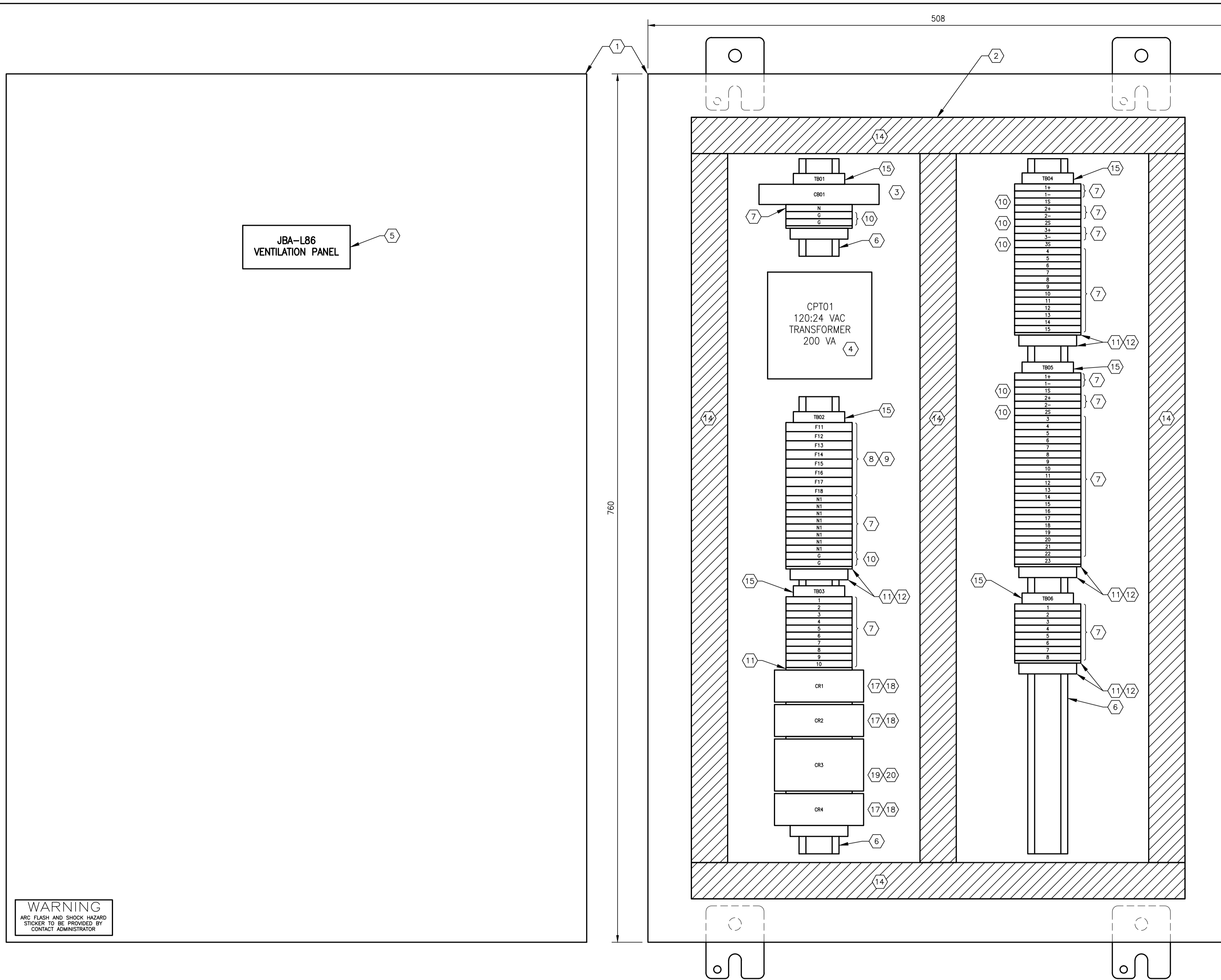
EXTERIOR PANEL VIEW SCALE: 1 : 2
