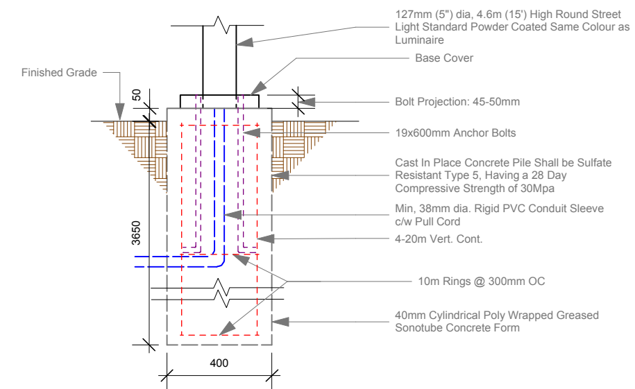
1 Lamp Standard Base Detail Scale: 1:20
