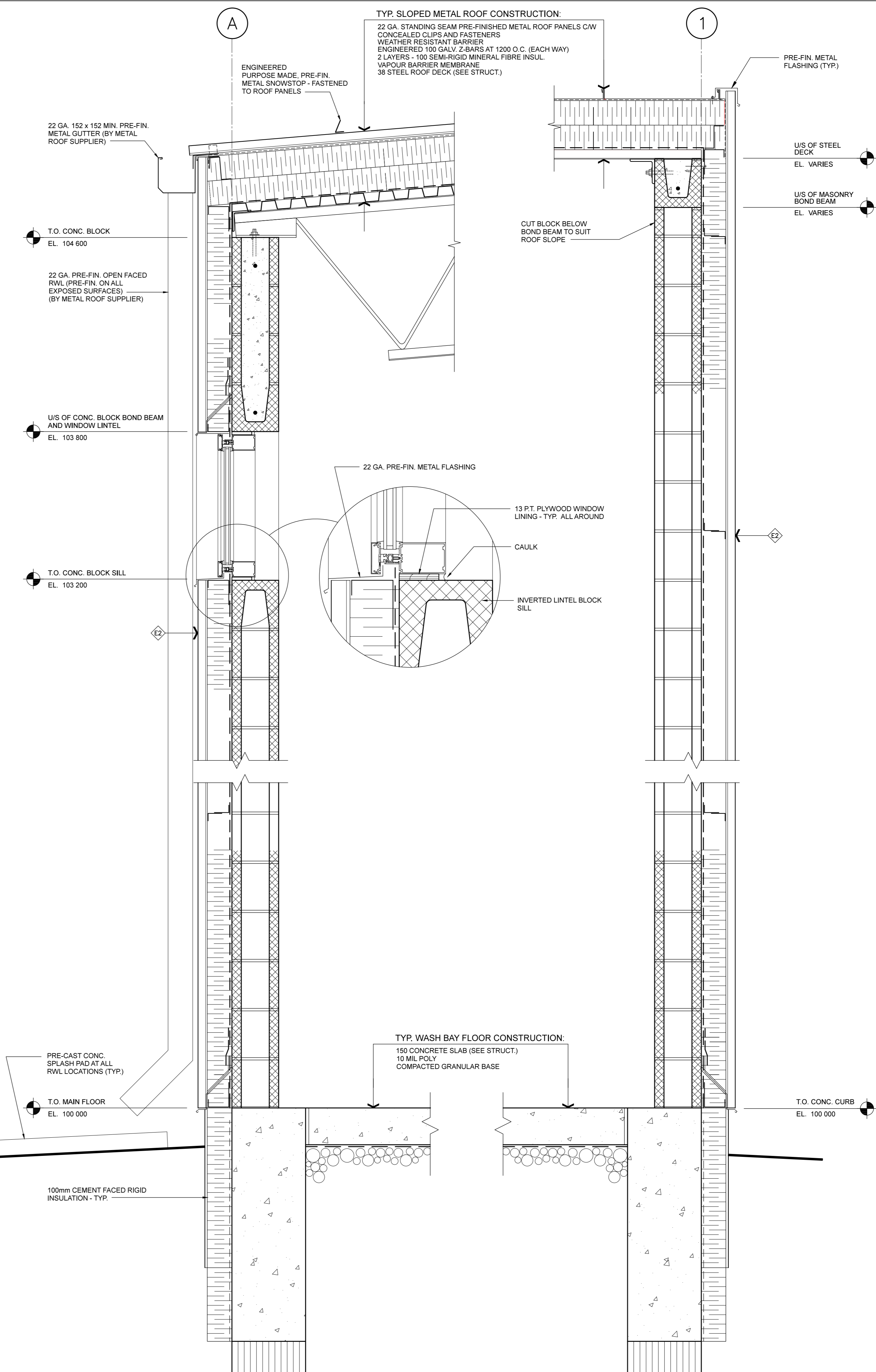
3 WALL SECTION A5.2 SCALE 1:10
