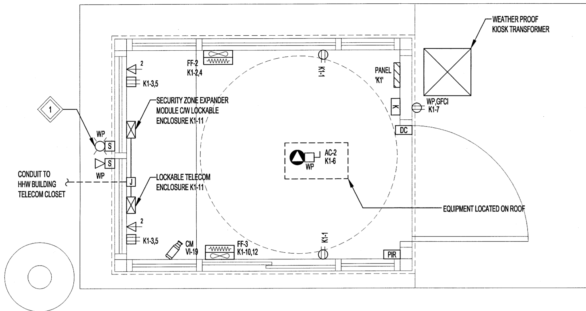
1 KIOSK #1 FLOOR PLAN - POWER & SYSTEMS SCALE: 1:20mm (24"x36")
