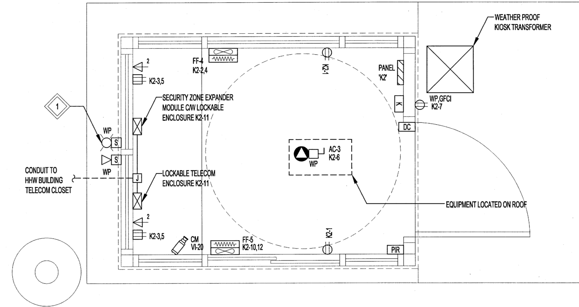
3 KIOSK #2 FLOOR PLAN - POWER & SYSTEMS SCALE: 1:20mm (24"x36")
