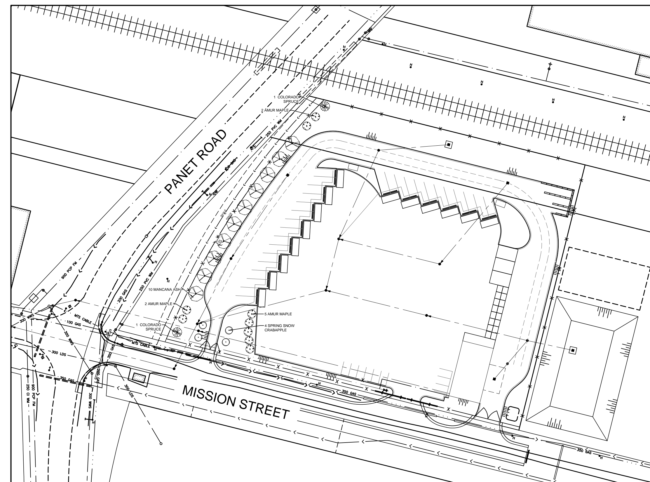
2 L1 CONTEXT PLAN SCALE - 1:1000 @ 24X36
