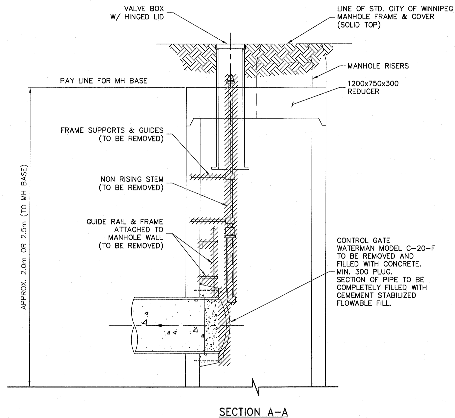
2 CONTROL GATE FOR OVERFLOWS TO STORM SEWERS NTS
