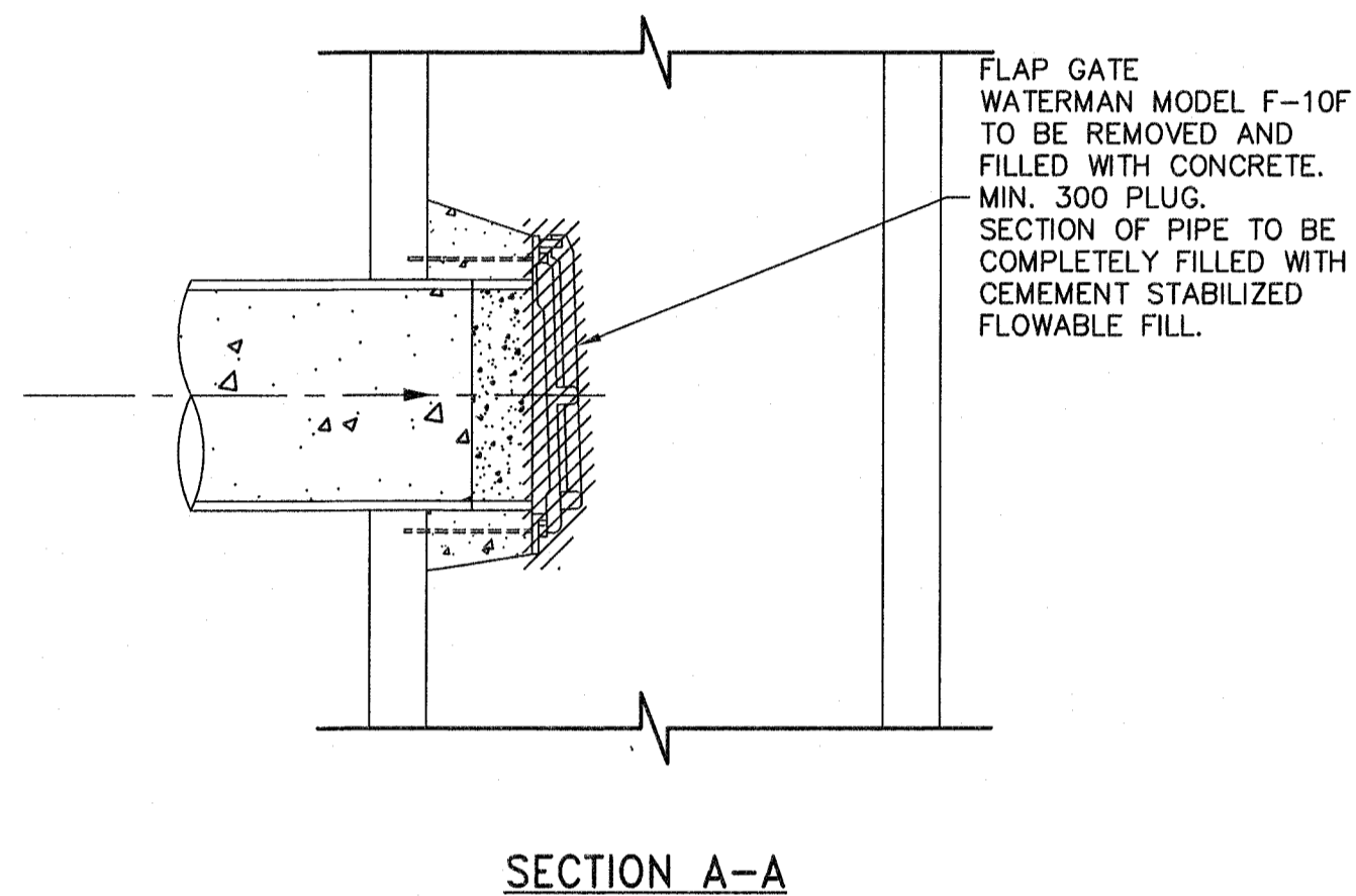
1 FLAP GATE IN EXISTING DMH NTS
