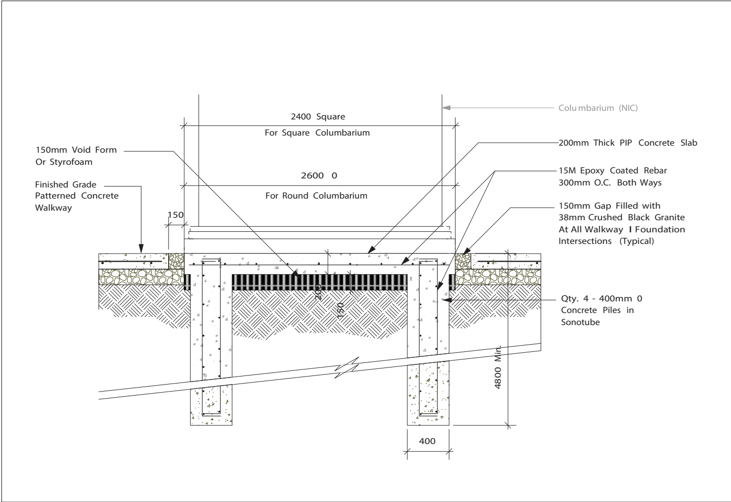
SQUARE / ROUND COLUMBARIUM FOUNDATION 1:25
