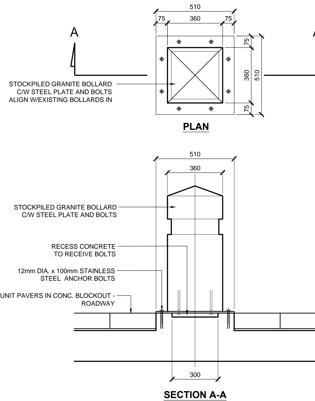
2 GRANITE BOLLARD FROM STOCKPILE SCALE 1:15
