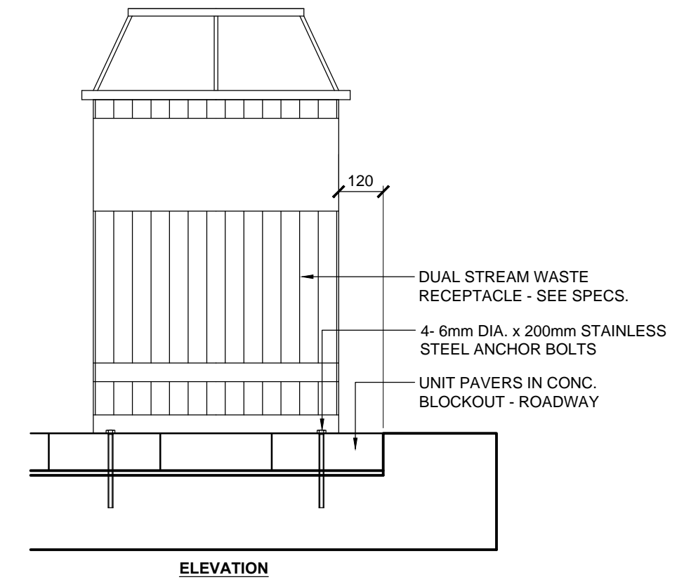
4 WASTE RECEPTACLE - SURFACE MOUNTED SCALE 1:15
