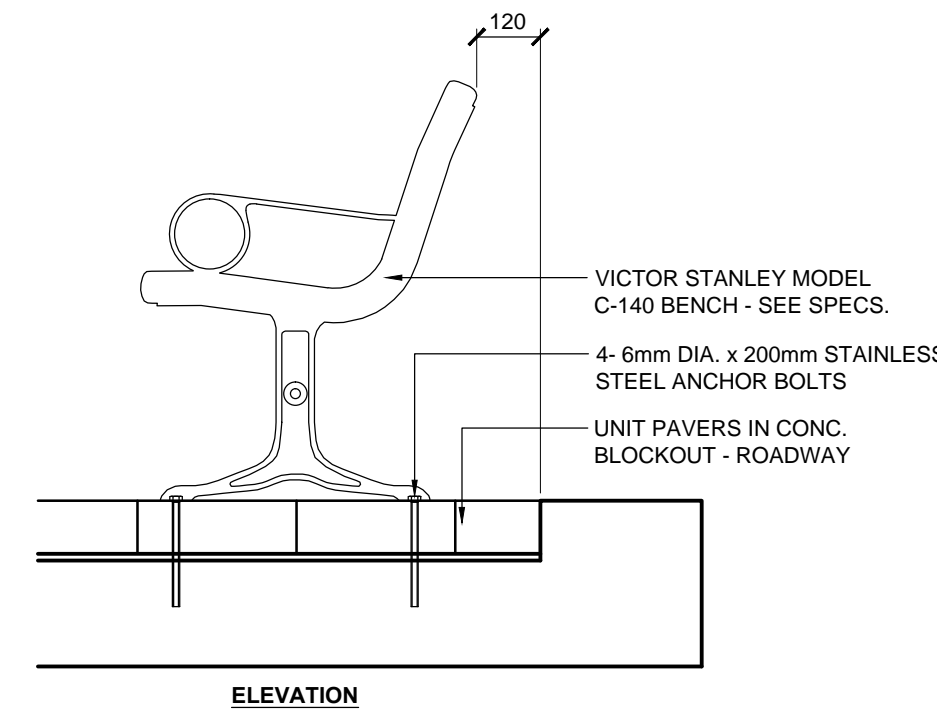
3 BENCH - SURFACE MOUNTED SCALE 1:15
