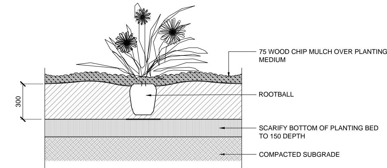
7 TYP. PERENNIAL / VINE PLANTING SCALE : NTS
