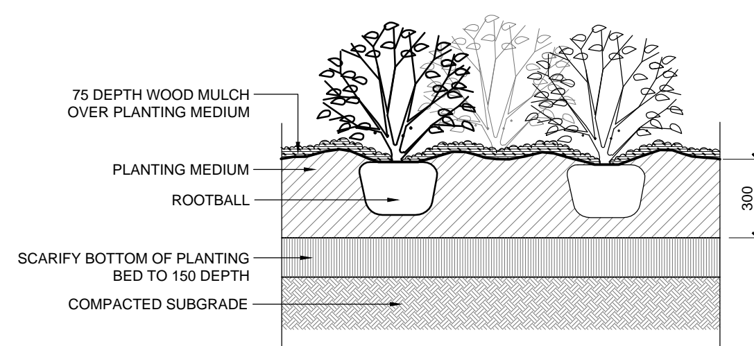
6 TYP. SHRUB PLANTING DETAIL SCALE : NTS
