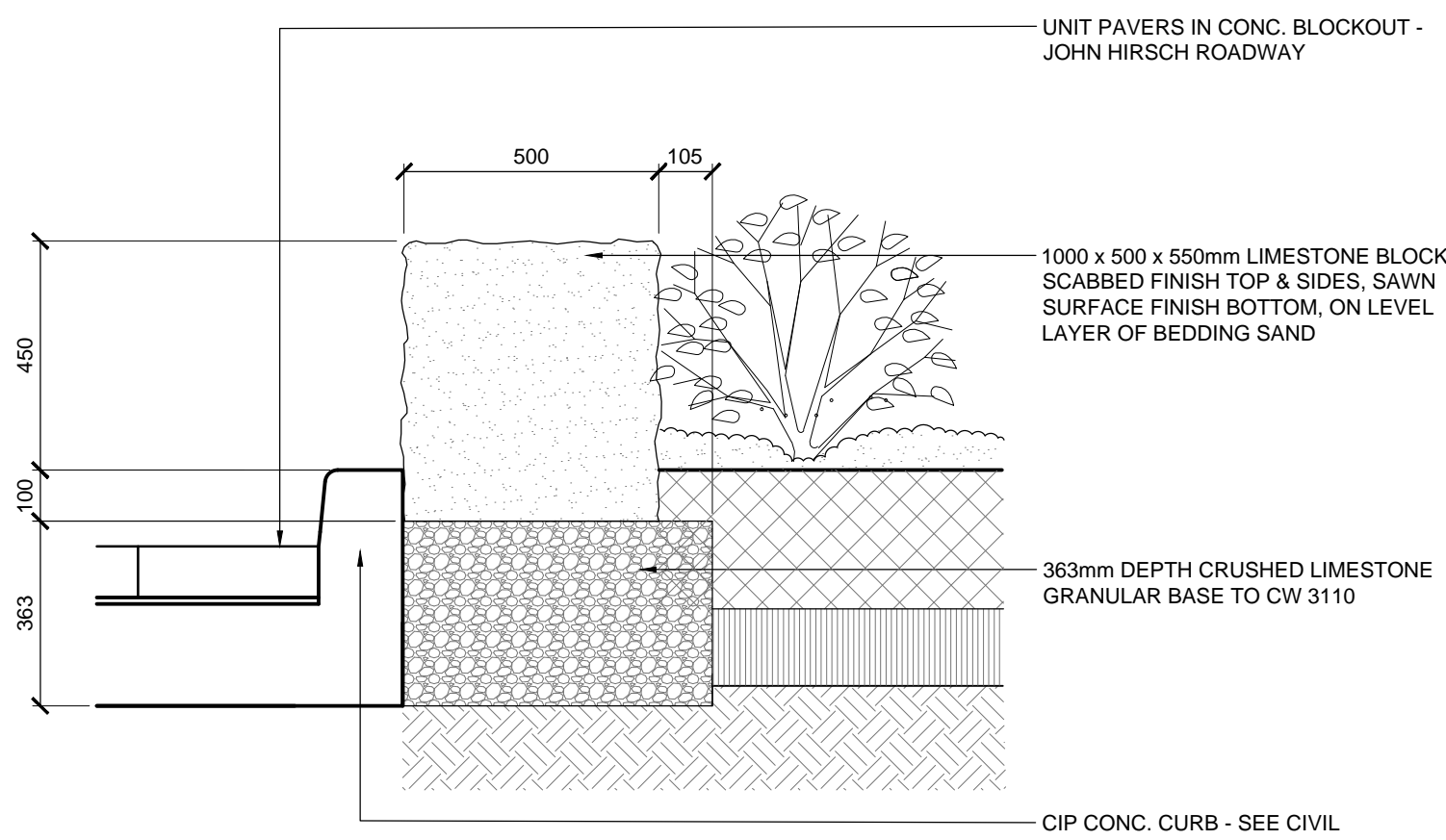
1 LIMESTONE BLOCK SCALE 1:15
