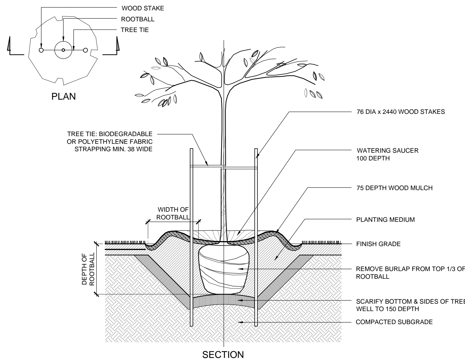
5 TYP. DECIDUOUS TREE PLANTING DETAIL SCALE : NTS
