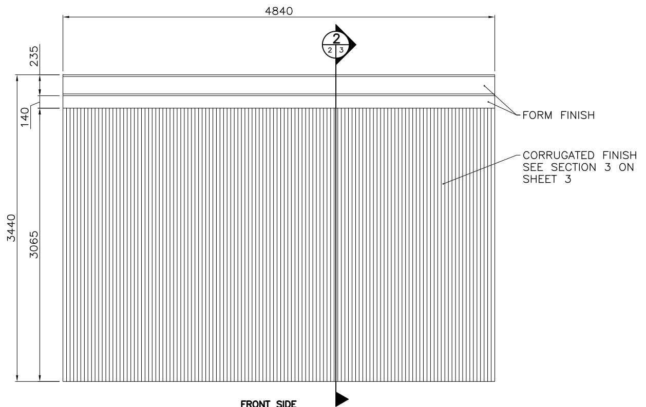
PANEL 2 ELEVATION NTS
