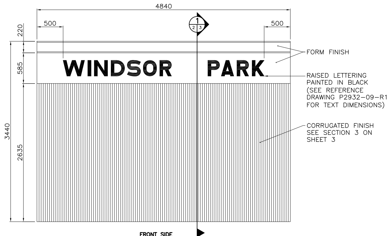
PANEL 1 ELEVATION NTS
