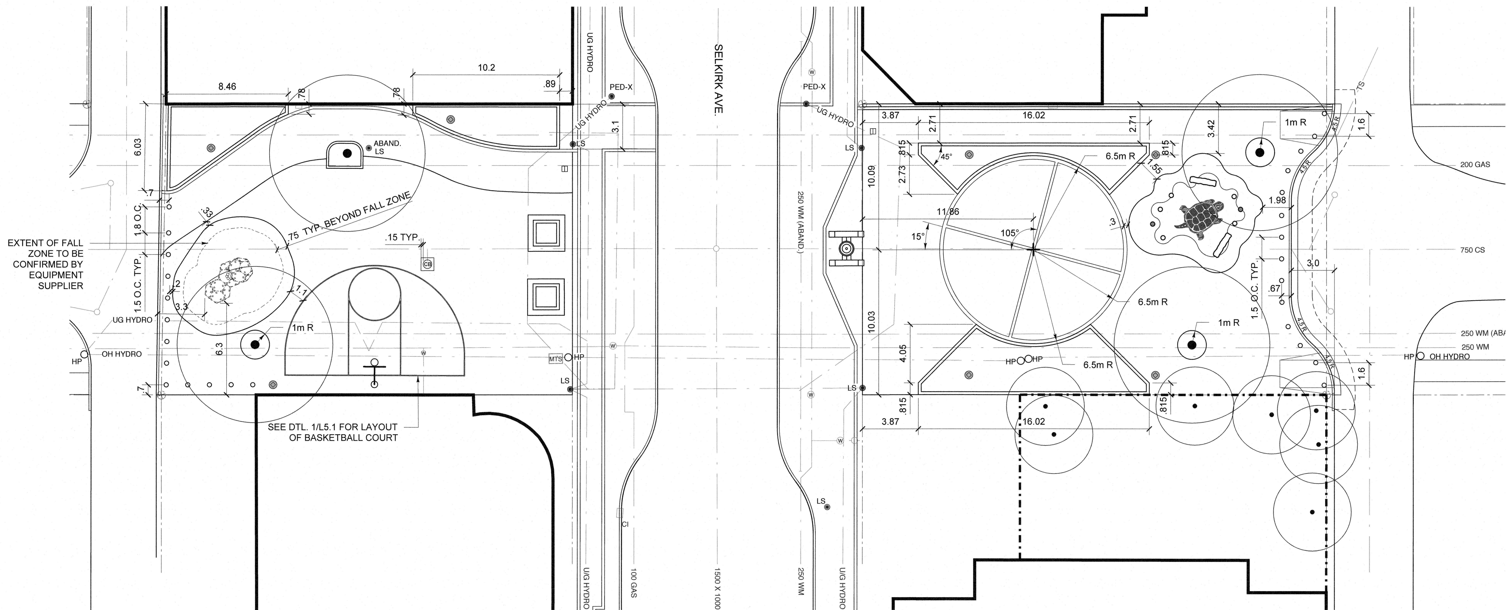
1 LAYOUT PLAN SCALE: 1:150 NORTH
