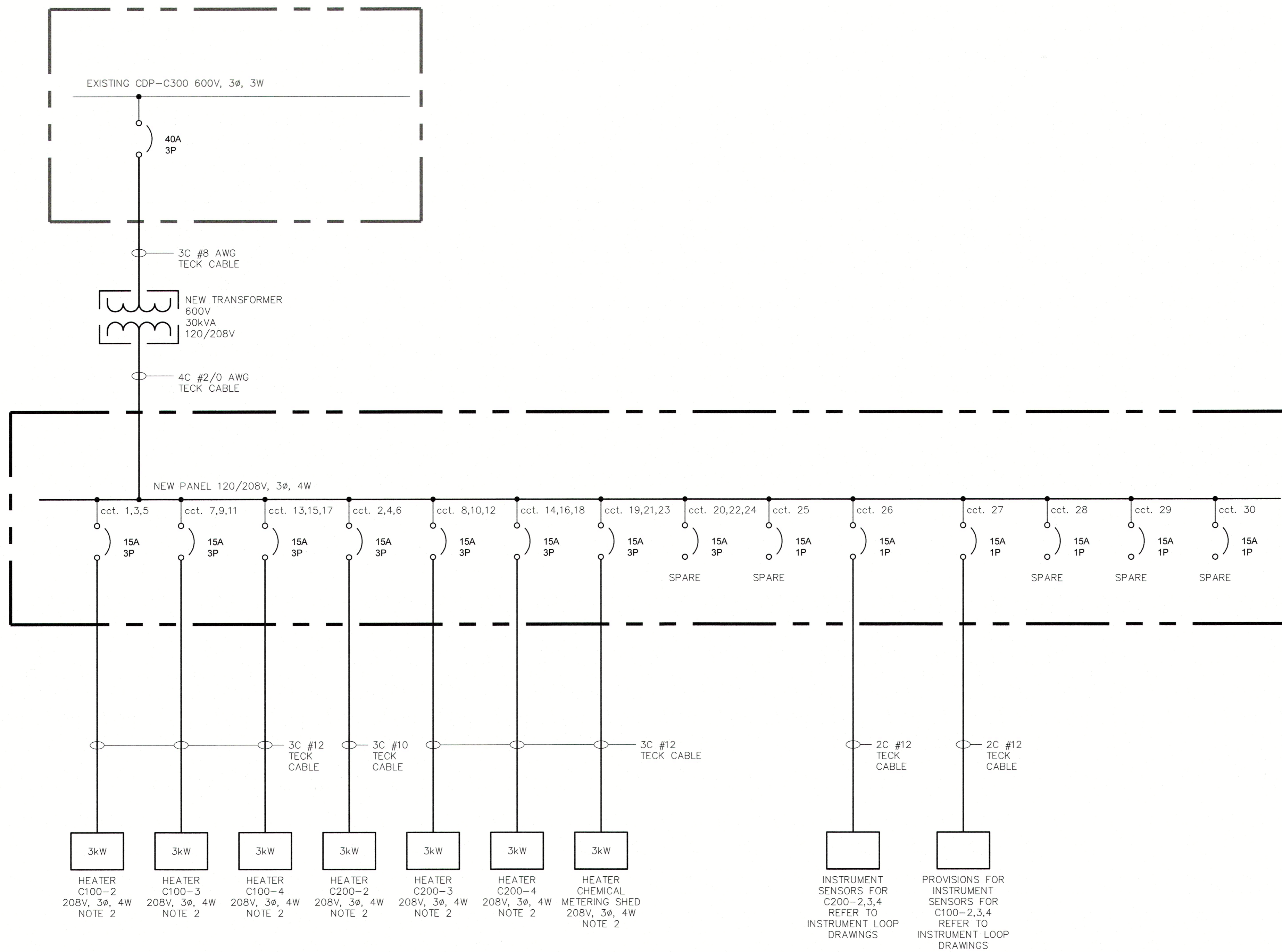
SINGLE LINE DIAGRAM SCALE : N.T.S.
