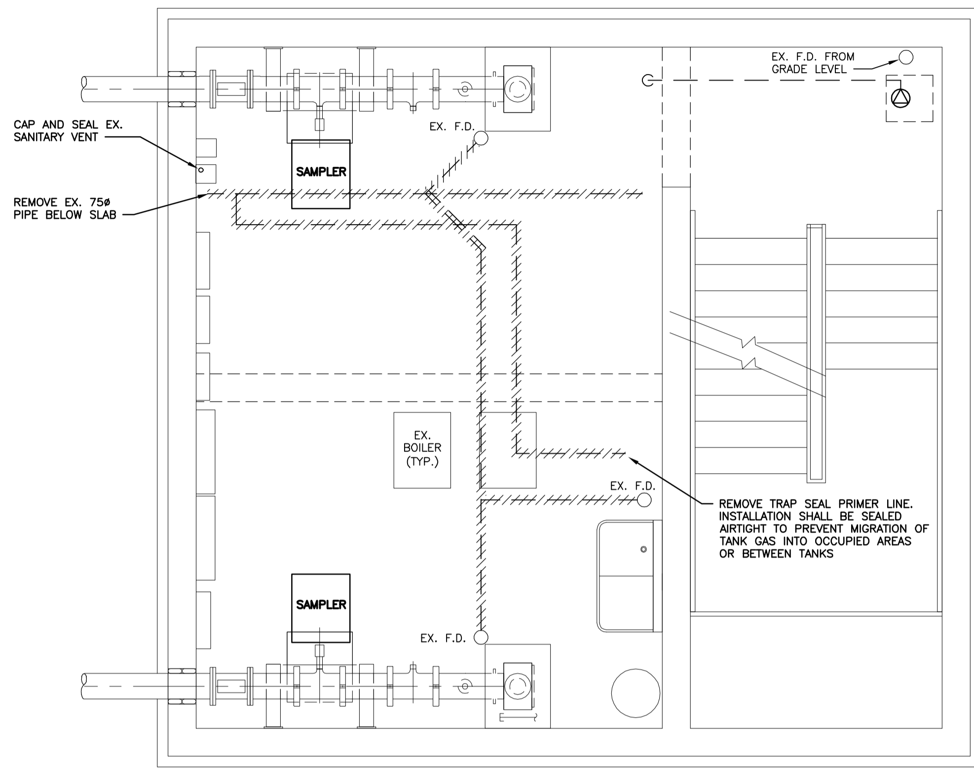
LEGEND // PIPE TO BE REMOVED 1 - DEMOLITION PLAN 1:40
