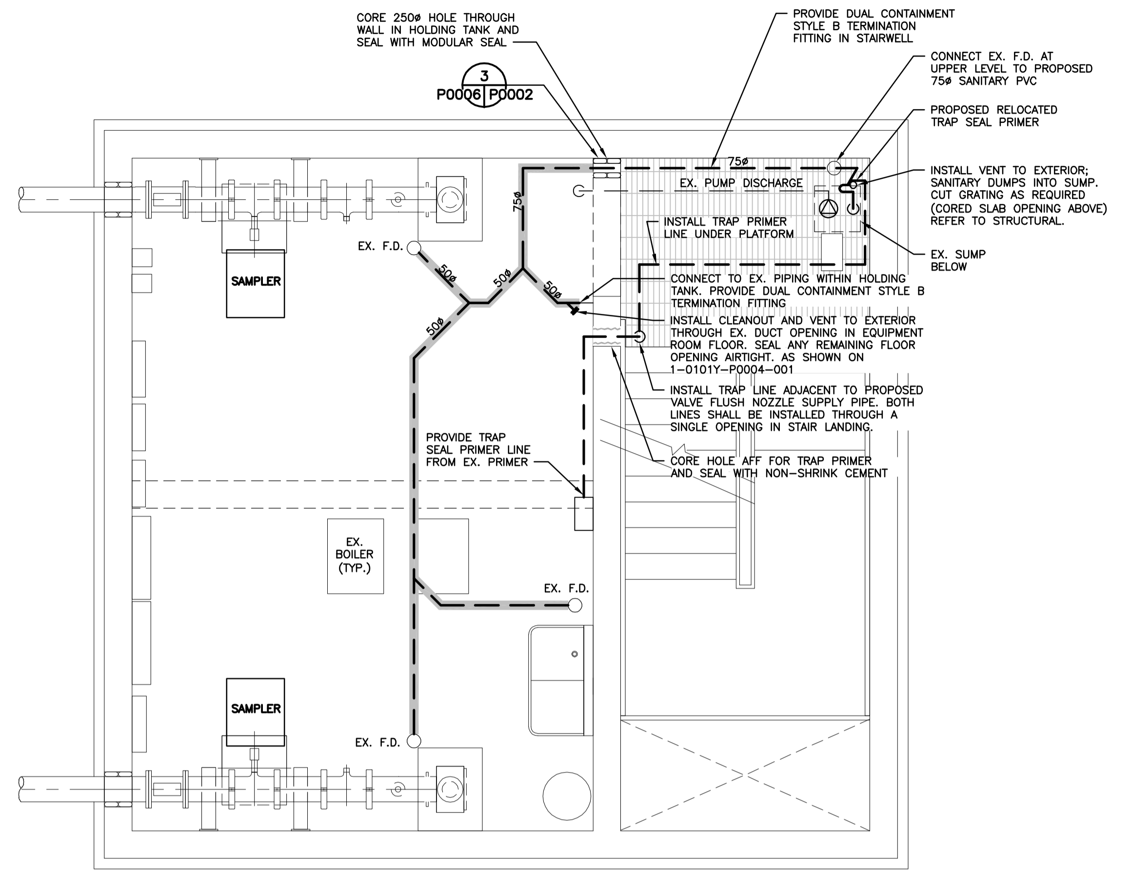
LEGEND --- DUAL CONTAINMENT PVC BELOW SLAB 2 - PROPOSED PLAN 1:40
