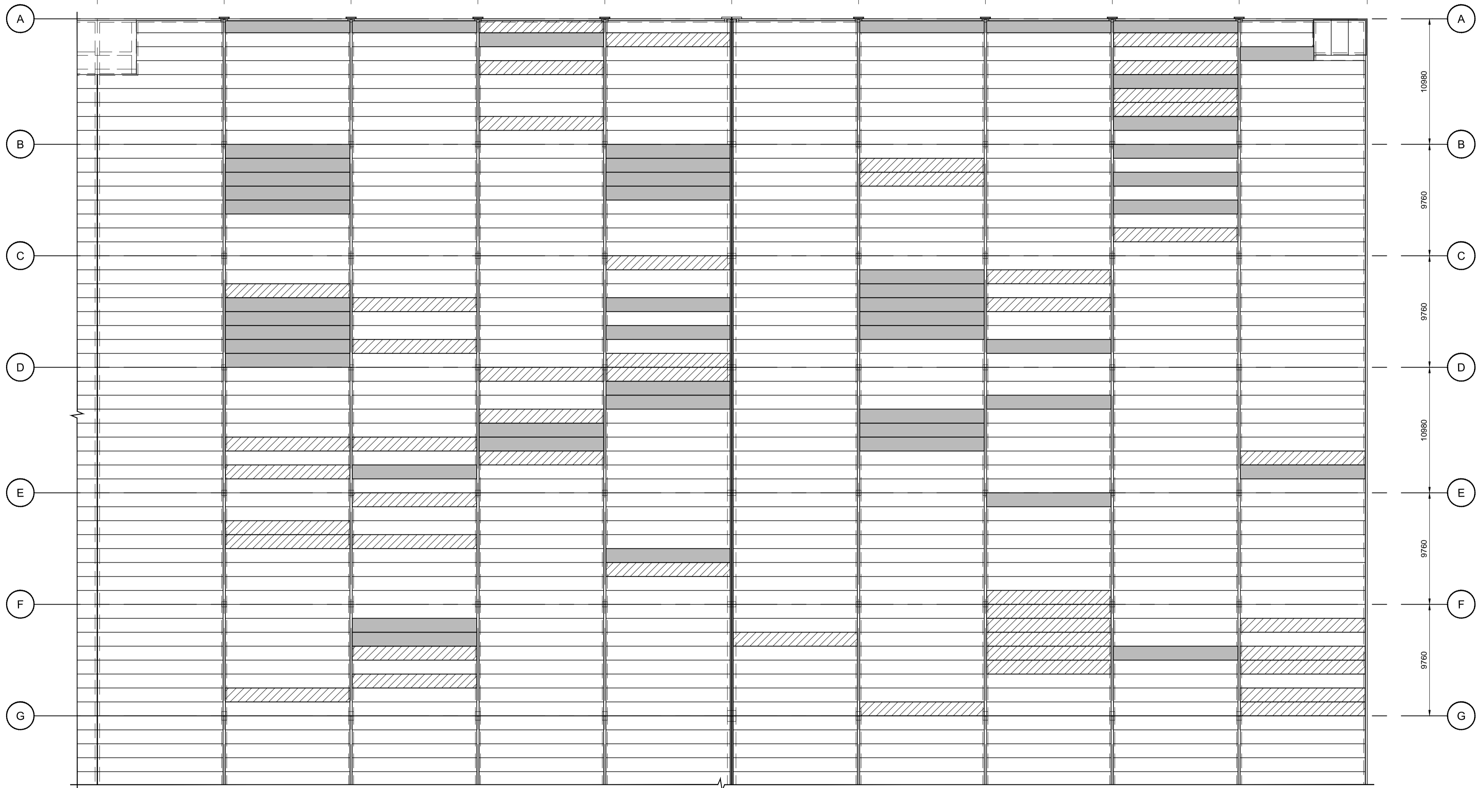
HOLLOWCORE REPLACEMENT PLAN, AREA "B" 1:200
