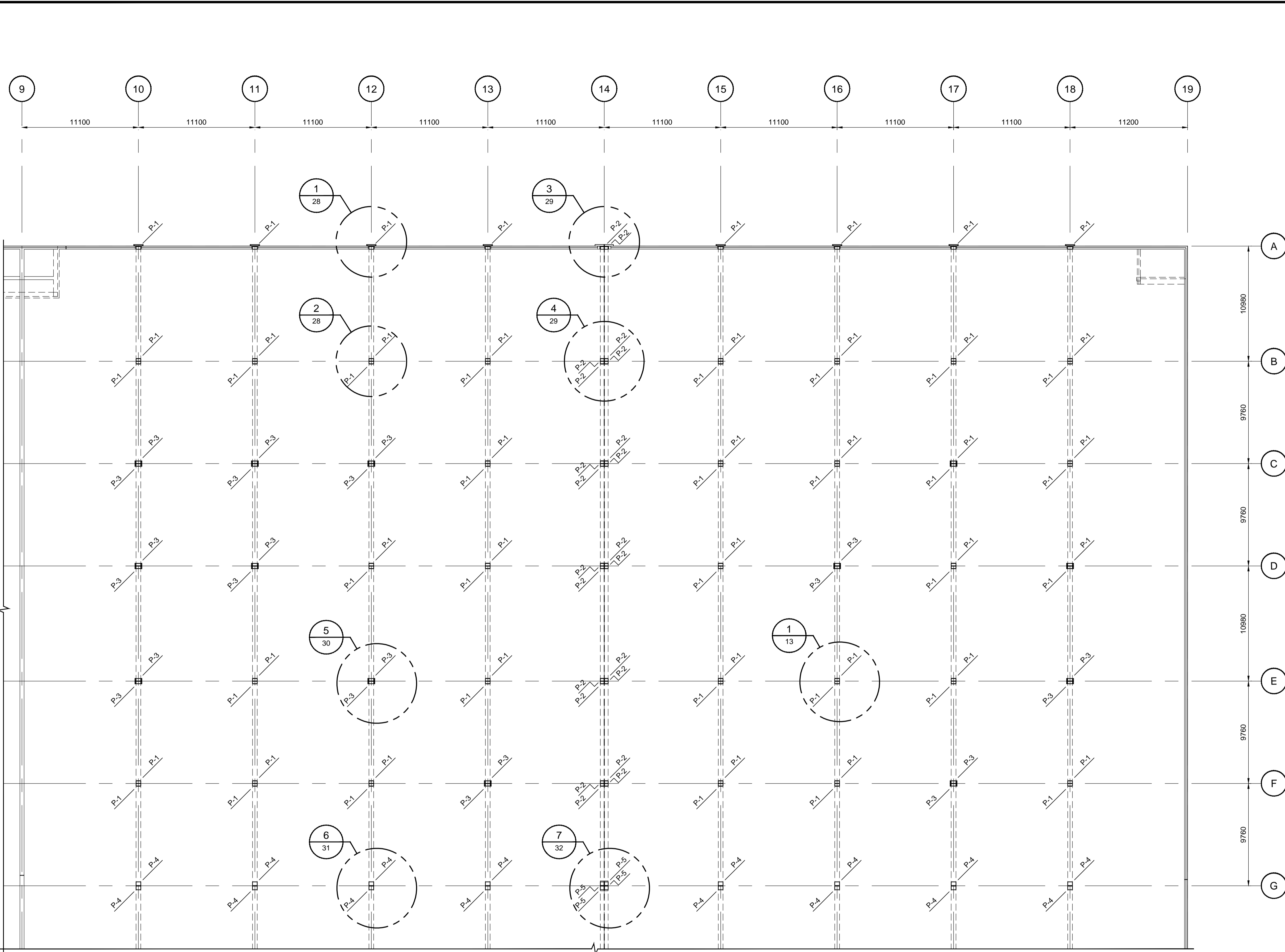
BEARING PLATE PLACEMENT PLAN, AREA "B" 1:200
