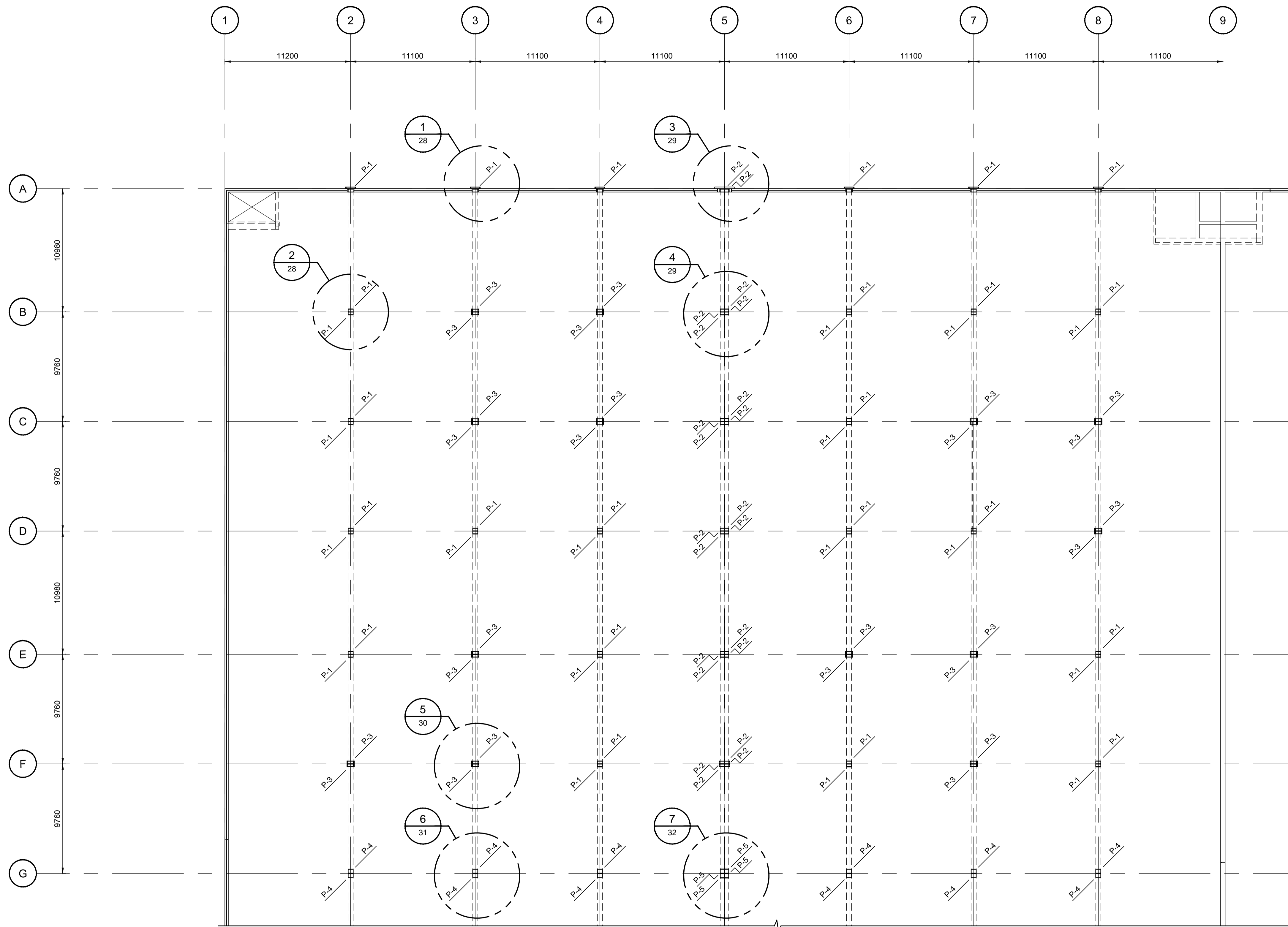
BEARING PLATE PLACEMENT PLAN, AREA "A" 1:200
