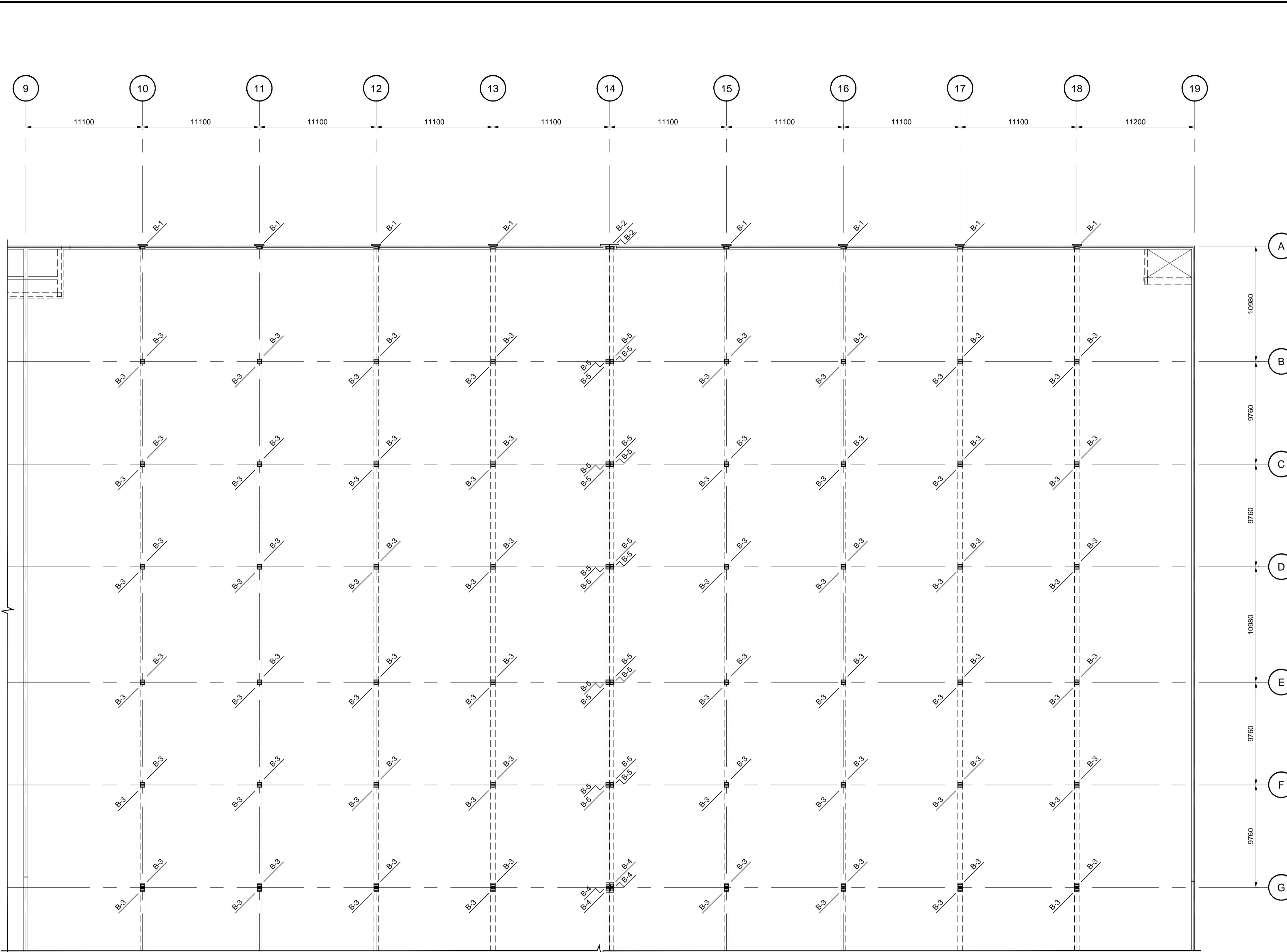
BEARING PAD REPLACEMENT PLAN, AREA "B" 1:200
