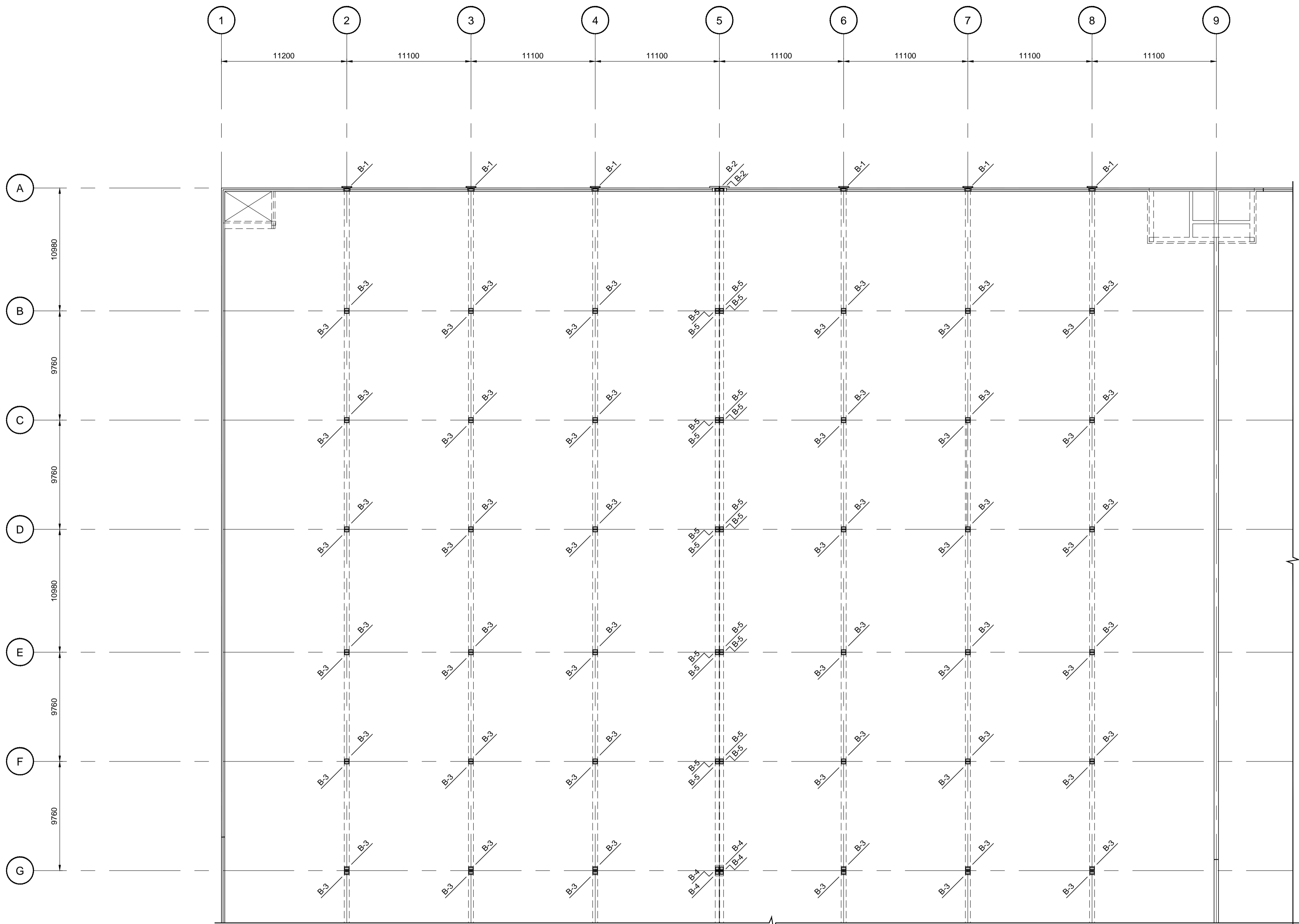
BEARING PAD REPLACEMENT PLAN, AREA "A" 1:200
