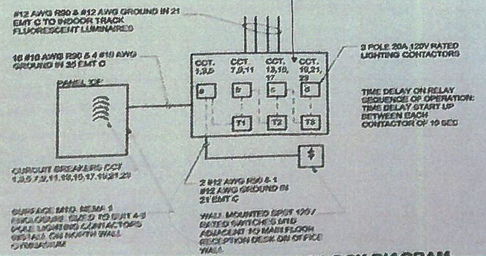
TRACK AREA LIGHTING CONTROL BLOCK DIAGRAM
