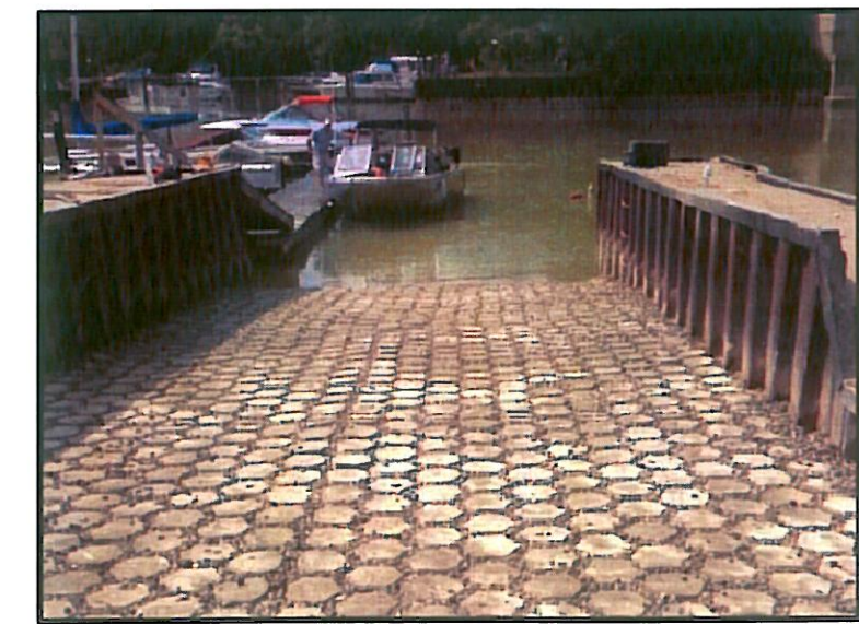
PHOTOGRAPH C: CABLE CONCRETE, CC G2 PRODUCT BOAT LAUNCH EXAMPLE.
