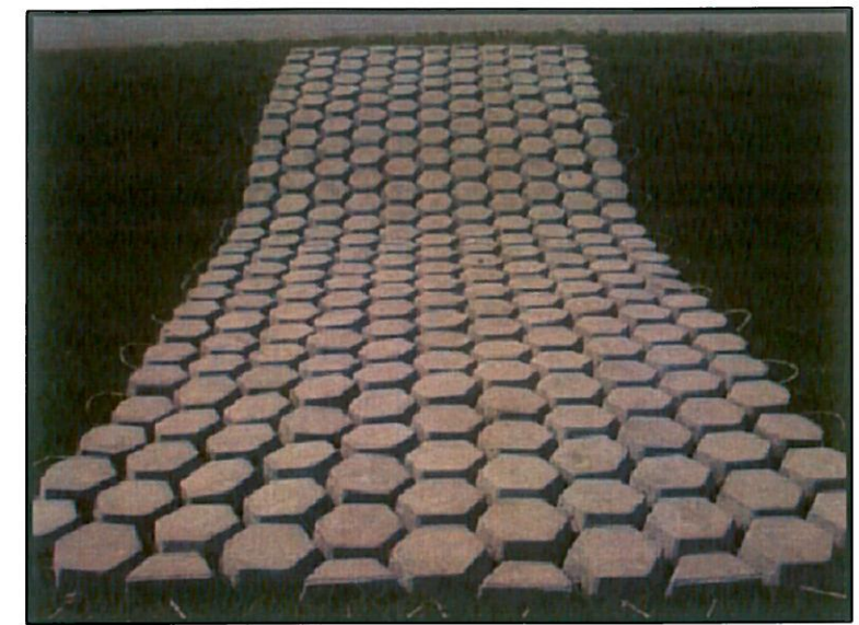
PHOTOGRAPH B: CABLE CONCRETE, CC G2 PRODUCT (TYP.).
