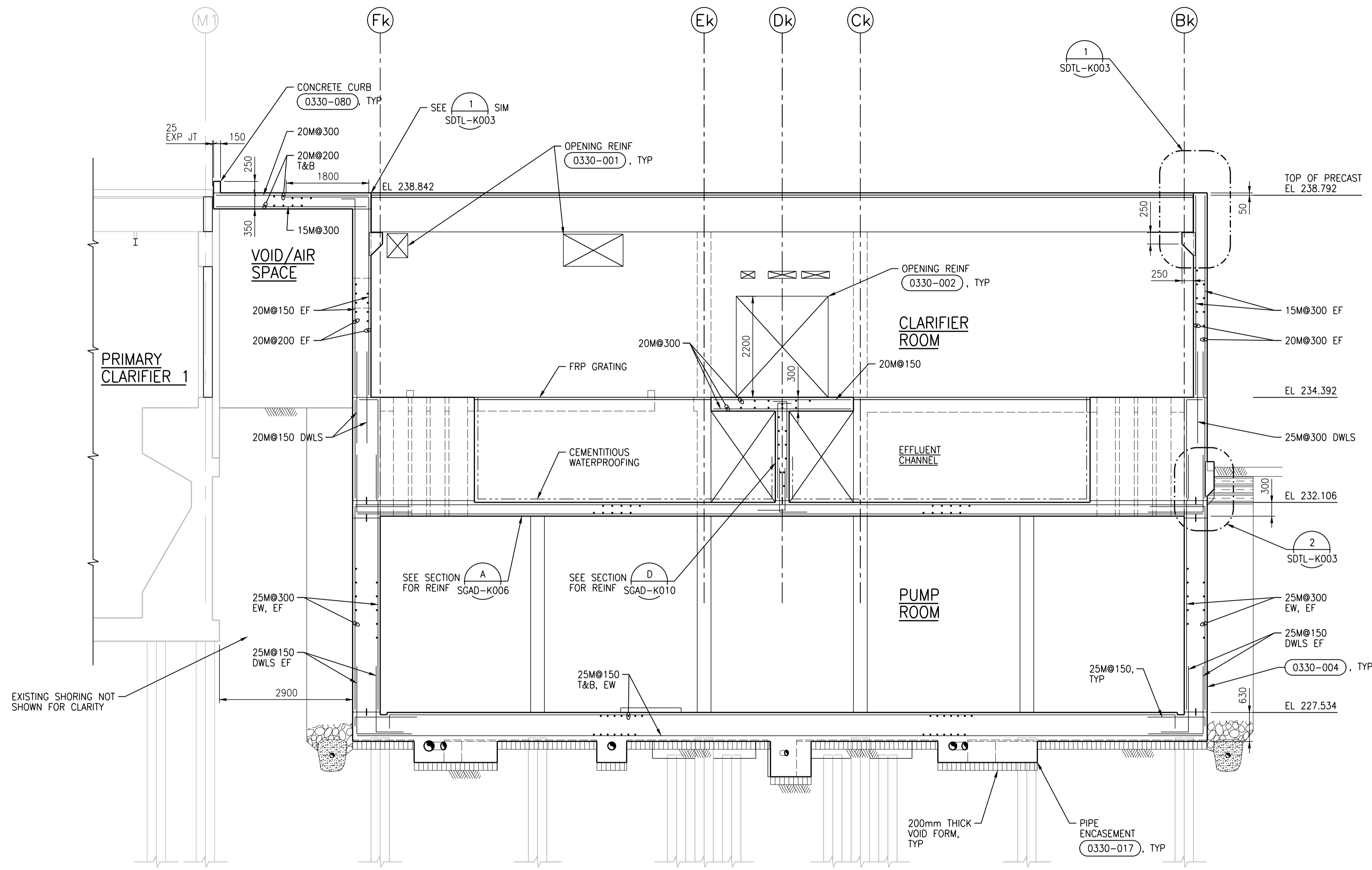
E SECTION 1:50 SGAD-K001, SGAD-K002, SGAD-K003, SGAD-K004
