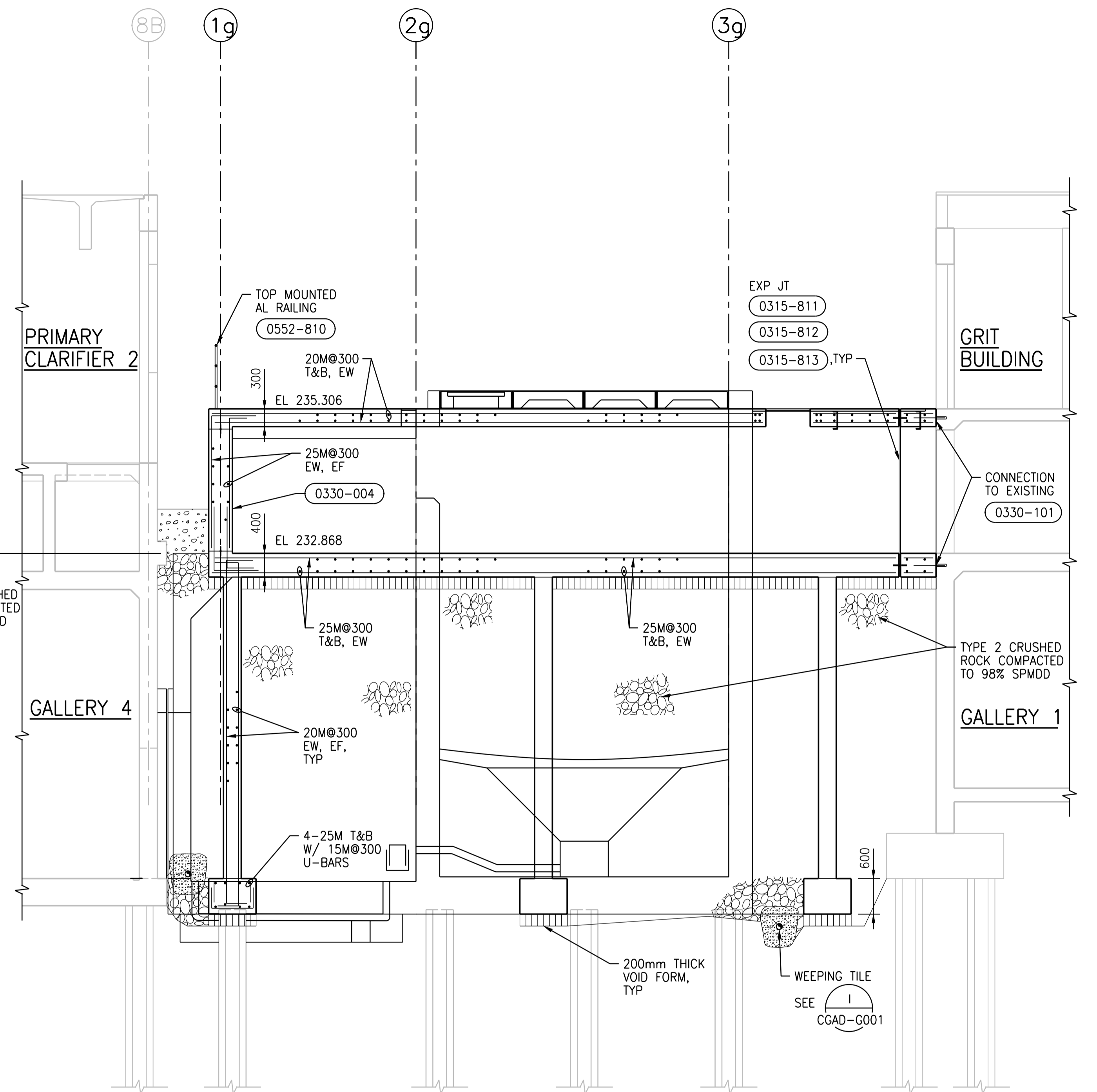
B SECTION 1:50 SGAD-G001, SGAD-G002, SGAD-G003
