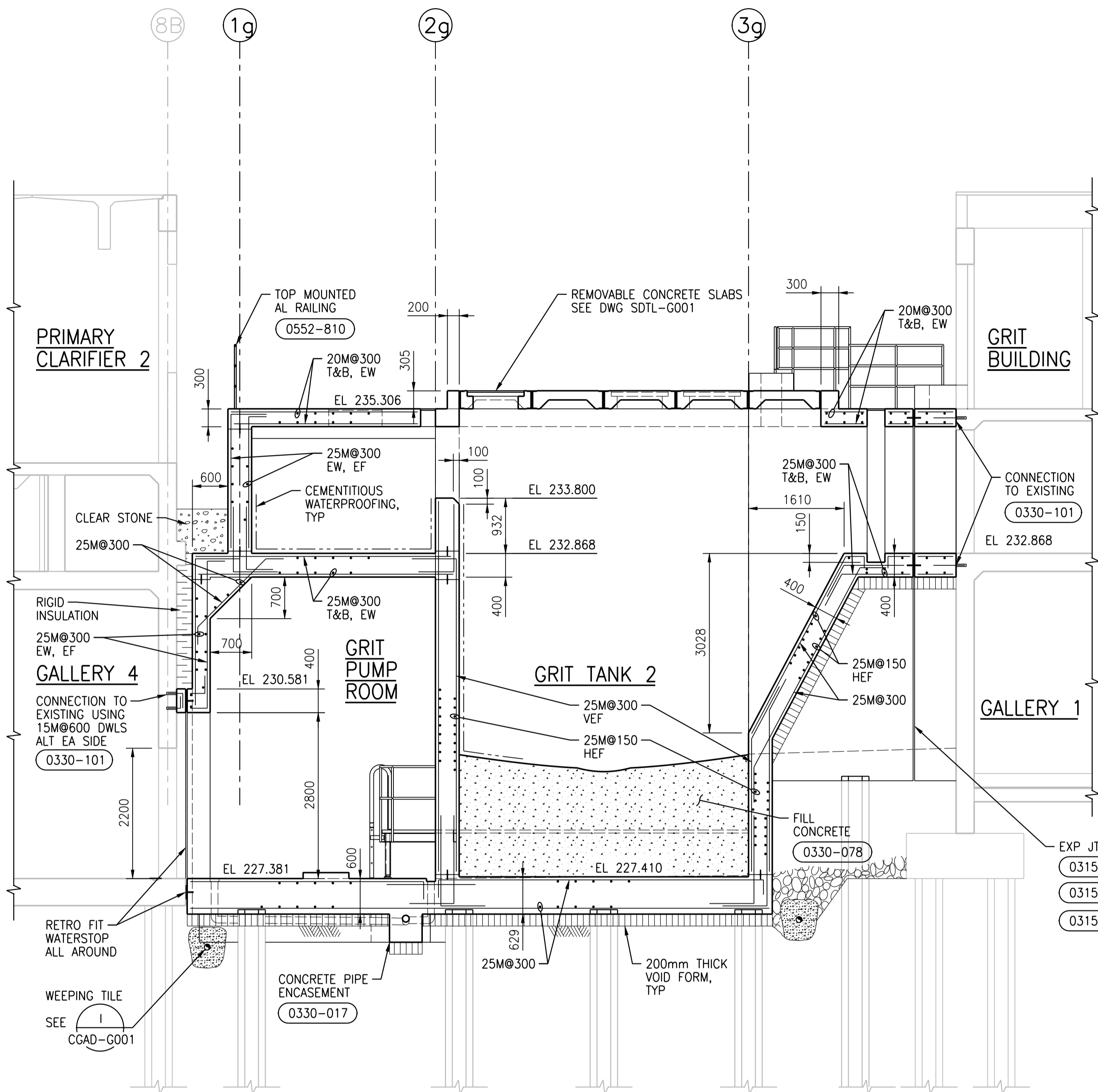
A SECTION 1:50 SGAD-G001, SGAD-G002, SGAD-G003
